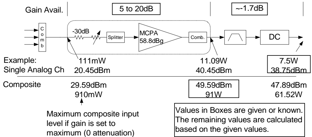
Figure C-1 Gain Block Example
