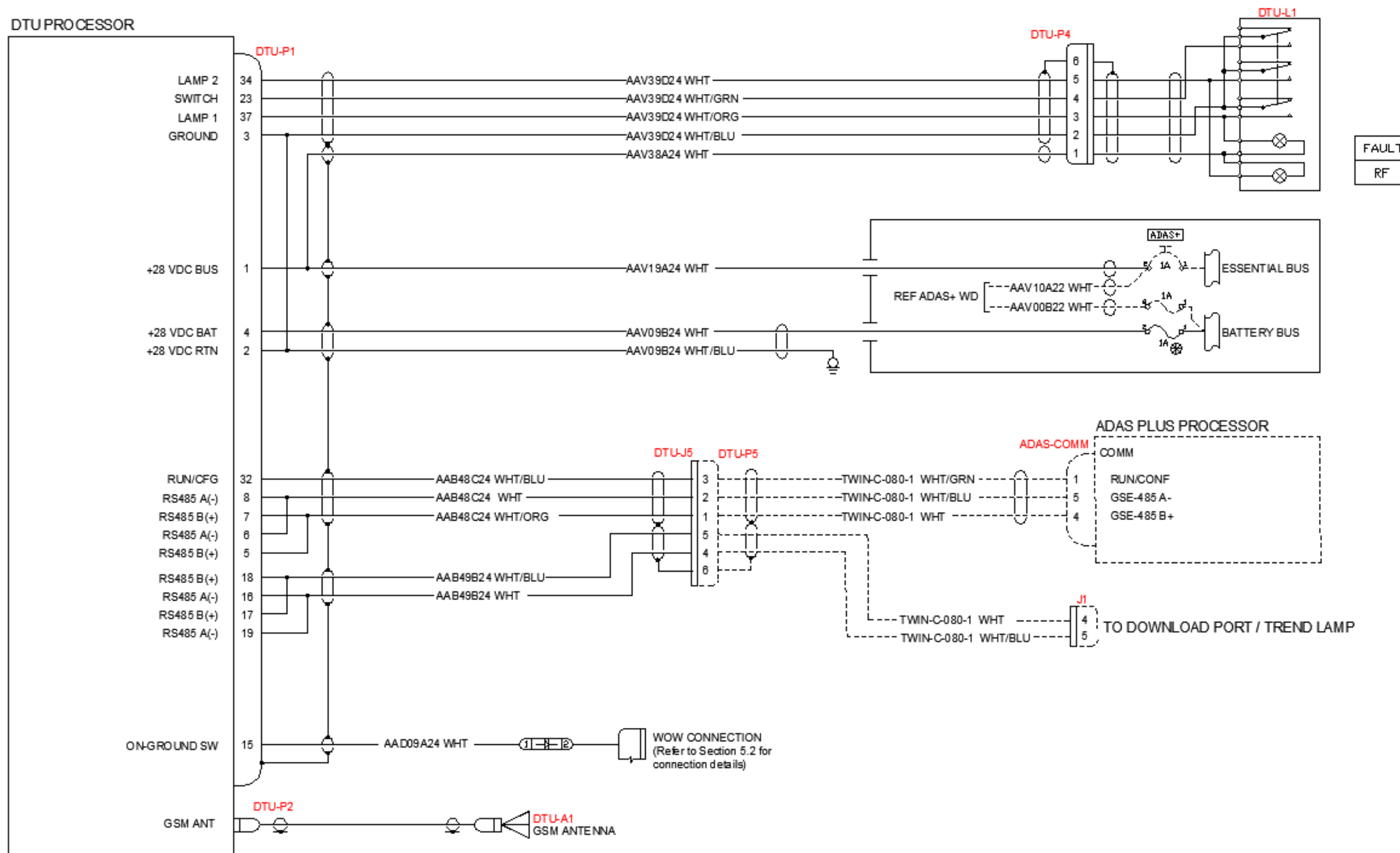
Figure B- 23: DTU / ADAS+ Upgrade Wiring Schematic
