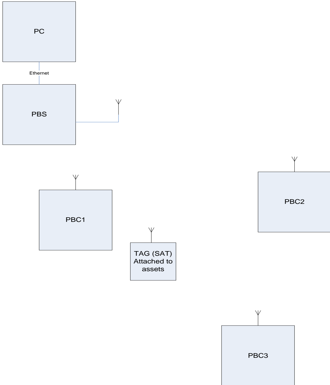
Figure 4 - iLocate system block diagram
