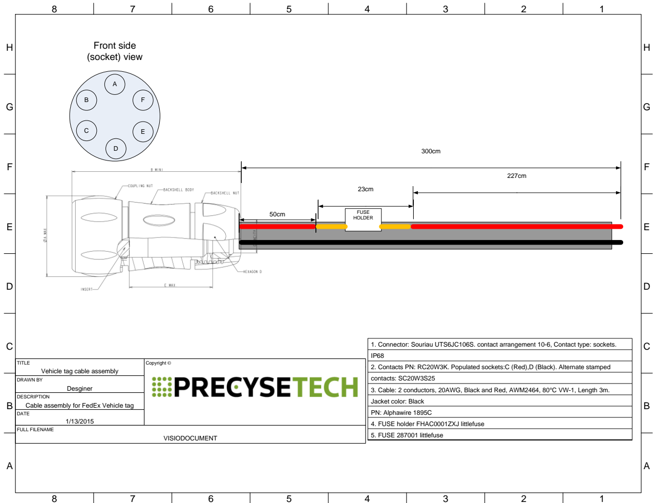
Figure 3 - optional cable with fuse
