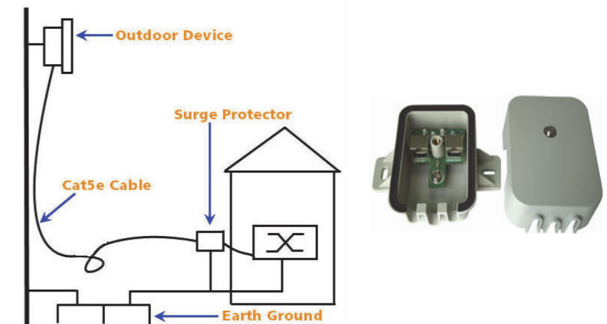
Figure 6: Surge Protector
