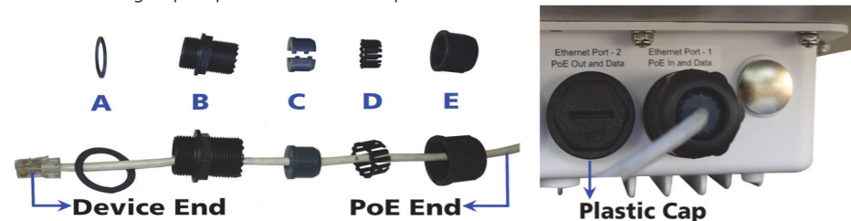
Figure 2: Weatherproofing RJ45 Connections
