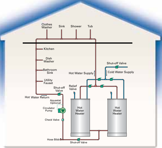
Multi-Story with 2 Water Heaters
