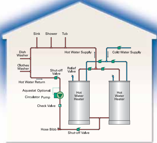
One-Story with 2 Water Heaters
