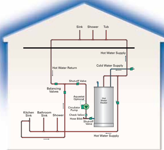
Multi-Story with 1 Water Heater
