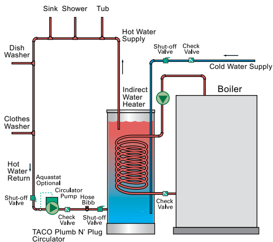
Recirculation Piping with Indirect Water Heater
