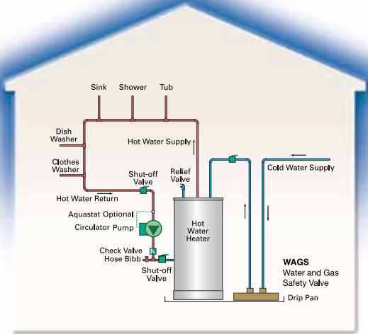
One-Story with 1 Water Heater
