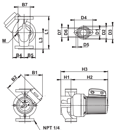
UP 43-70 F
