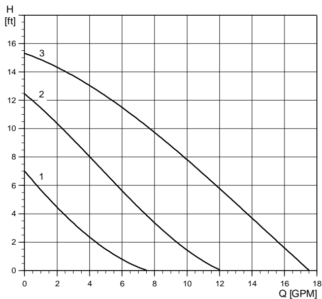
UPS 15-42 F
