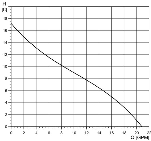
UP 15-55 SUC
