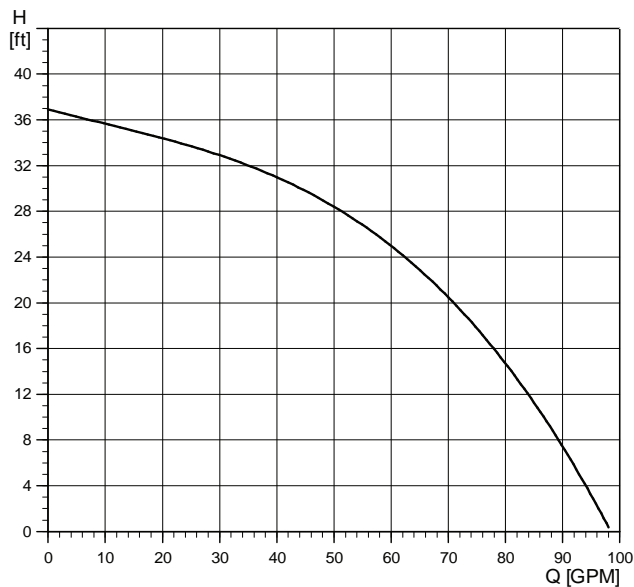
UP 43-110 F
