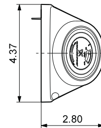
Fig. 3 Timer dimensions, current version
