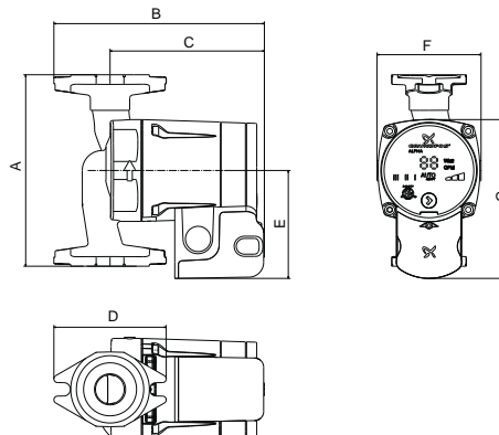
ALPHA 15-55 FR Terminal box
