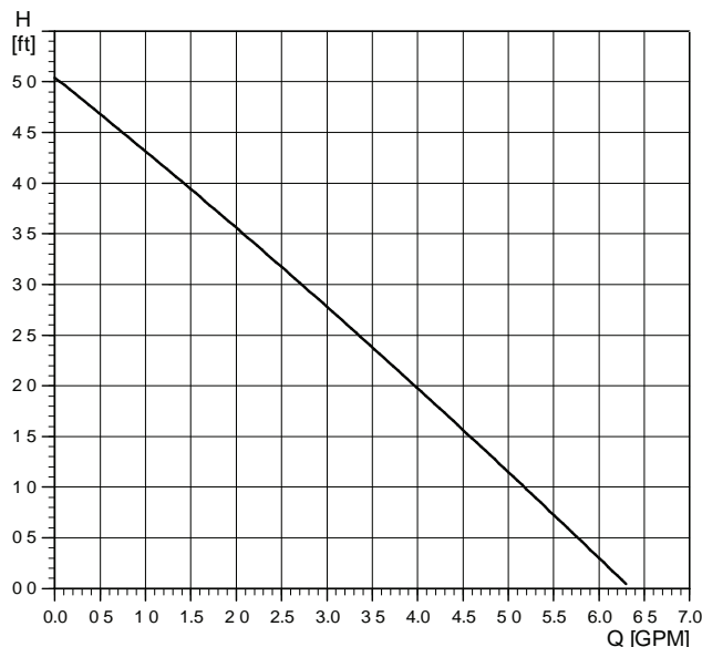
UP 15-10 SU7P/TLC
