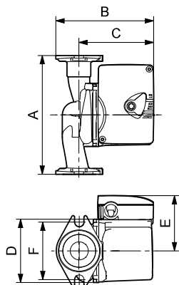
UPS 15-55 SFC
