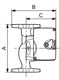
UPS 15-58 FRC
