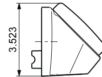
Fig. 2 Timer dimensions, previous version
