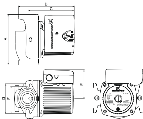
UPS 26-150 F/SF
