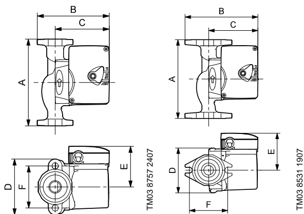
UPS 26-99 FC
