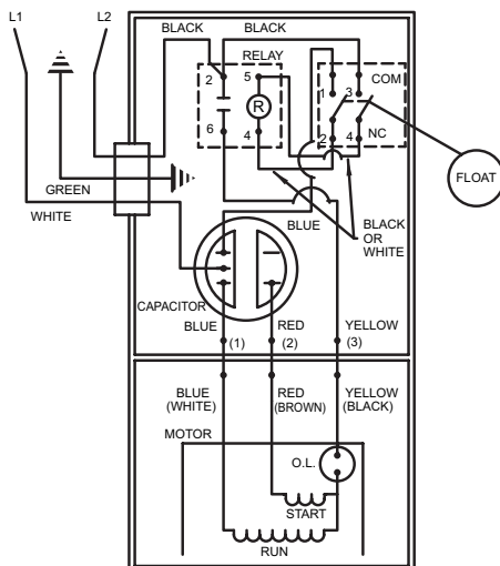
WIRING DIAGRAM FOR MODELS "M292" All Revisions 1/87 (MT) thru Current
