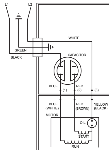
WIRING DIAGRAM FOR MODELS "N294" All Revisions 1/87 (MT) thru Current
