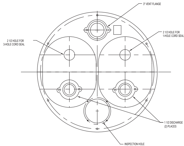
FIG. 3 24" COVER
