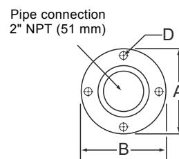
Isolating valve GU 125 union
