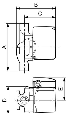
UP 15-10 B5 and UP 15-10 B5/LC
