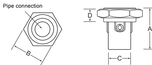
Isolating valve GU 125 union
