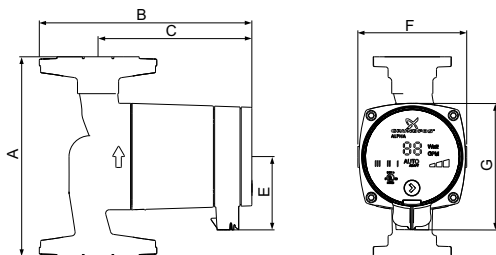
ALPHA 15-55 FR line cord
