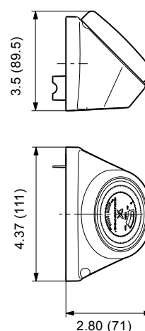
Fig. 13 Timer dimensions, current version
