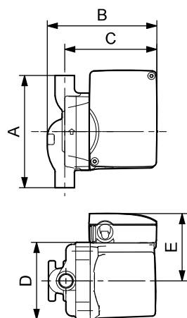
UP 15-10 B5 and UP 15-10 B5/LC
