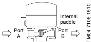
Fig. 3 Two-way valve, normally closed
