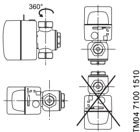
Fig. 1 Valve body installation
