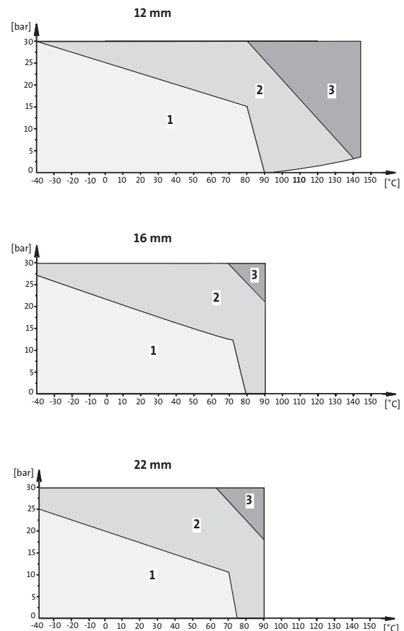
Fig. 49 Pressure-temperature diagrams
