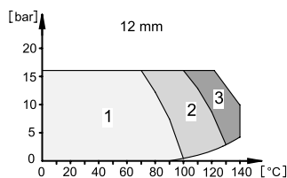
Fig. 33 Pressure-temperature diagrams
