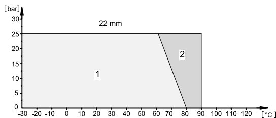
Fig. 41 Pressure-temperature diagram
