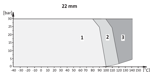
Fig. 46 Pressure-temperature diagrams
