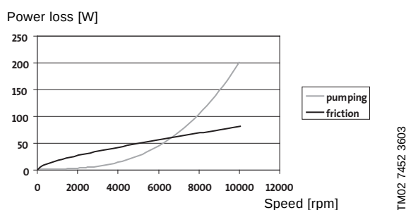
Fig. 11 Power consumption of seal
