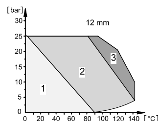
Fig. 31 Pressure-temperature diagrams
