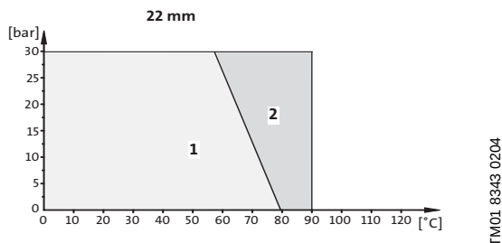
Fig. 52 Pressure-temperature diagram
