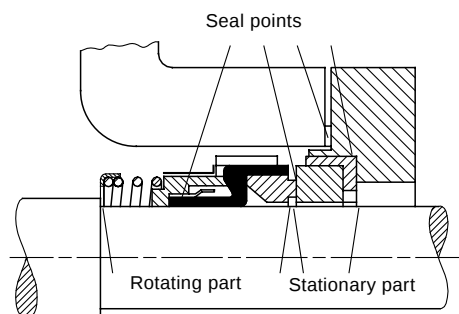
Fig. 5 Main components of a mechanical shaft seal
