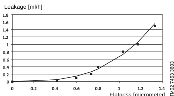
Fig. 13 Flatness as a function of leakage
