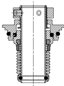
Fig. 50 Type K seal
