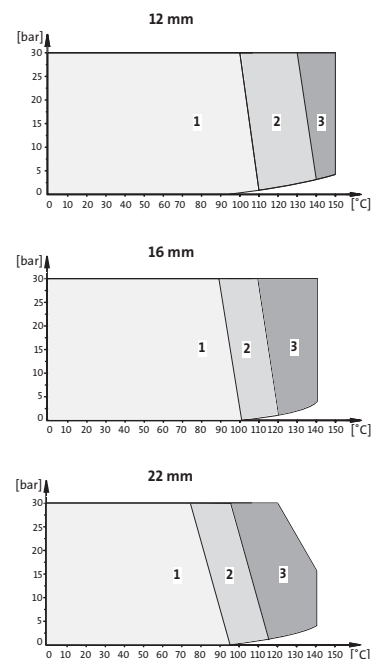
Fig. 48 Pressure-temperature diagrams
