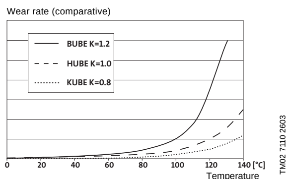
Fig. 12 Wear rate for different balancing ratios
