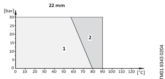
Fig. 53 Pressure-temperature diagram
