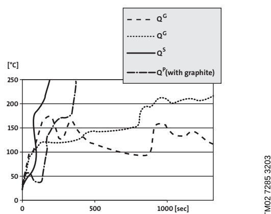
Fig. 25 Dry-running performance of seals
