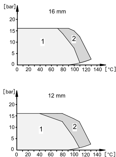
Fig. 34 Pressure-temperature diagram
