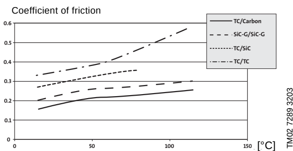
Fig. 29 Start friction in water
