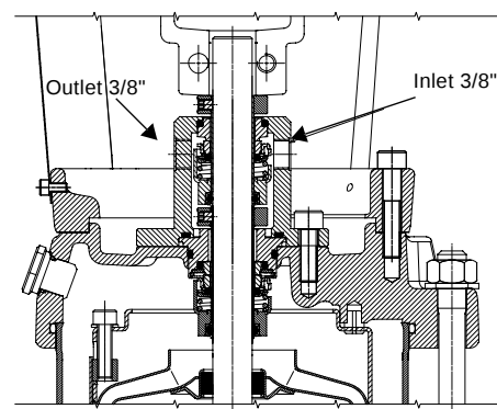
Fig. 57 Tandem seal arrangement in a CR pump
