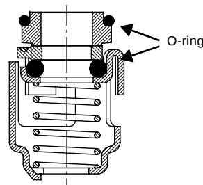
Fig. 15 O-ring shaft seal
