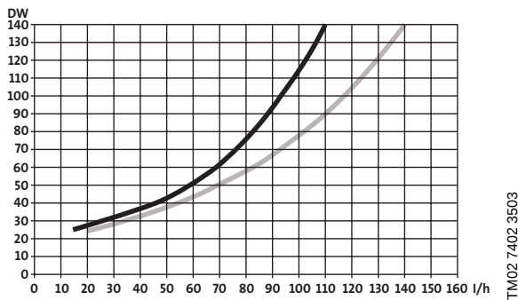
Fig. 62 Circulation volume of Cartex-DE
