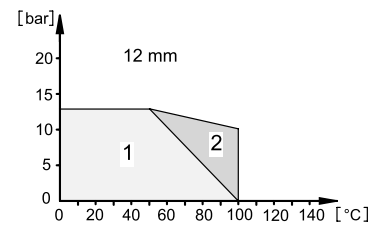
Fig. 37 Pressure-temperature diagram
