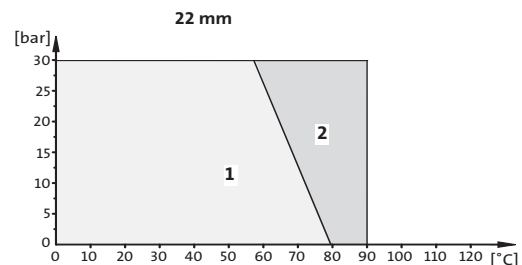
Fig. 40 Pressure-temperature diagram
