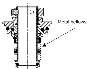
Fig. 17 Metal bellows shaft seal
