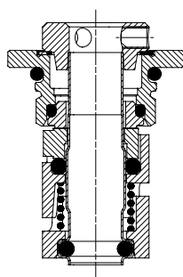
Fig. 45 Type H seal
