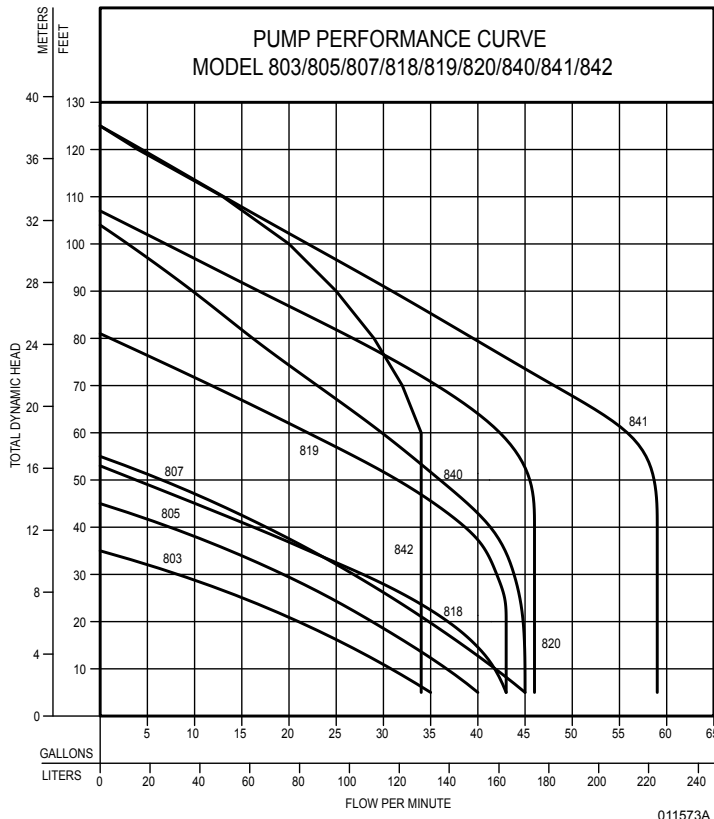
TOTAL DYNAMIC HEAD/FLOW PER MINUTE SEWAGE
