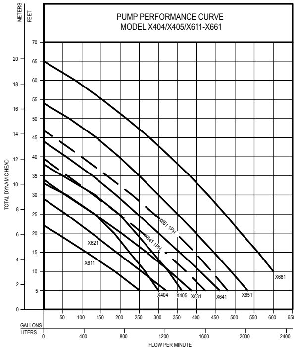
TOTAL DYNAMIC HEAD/FLOW PER MINUTE SEWAGE
