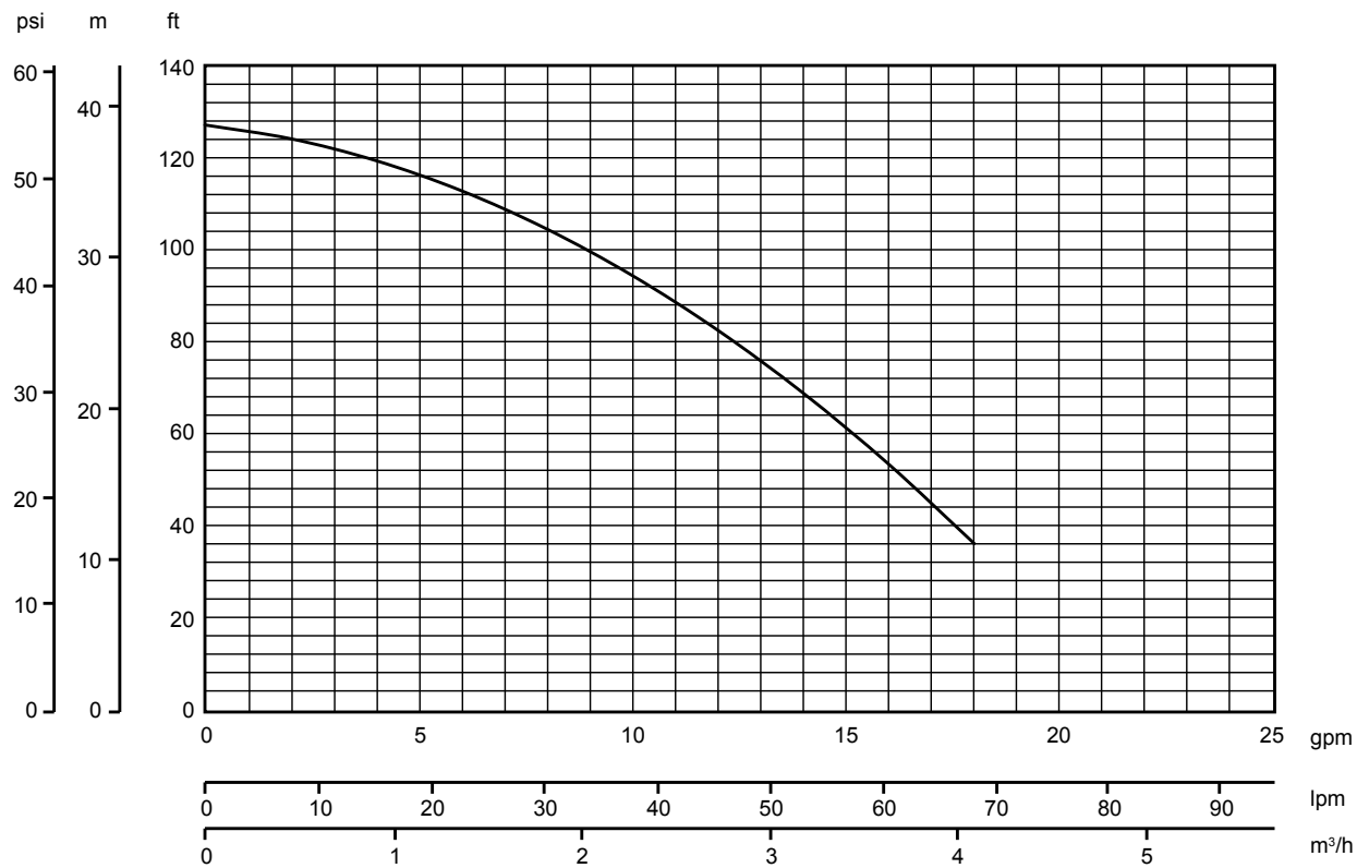
Appendix 1: Inline Pressure Boosting System Performance Curve (60 Hz)
