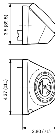
Fig. 13 Timer dimensions, current version
