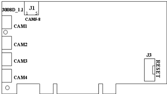
Figure2-1 TD3008 Video Capture Card
