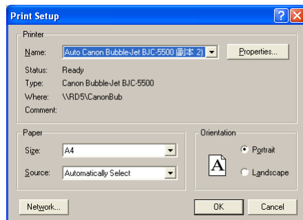
Figure7-15Print Setup
