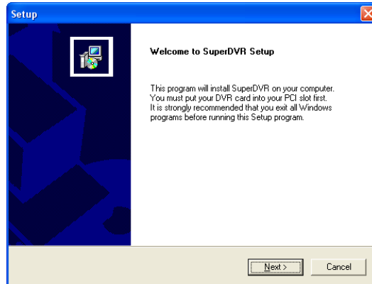
Figure3-7 Welcome Page
