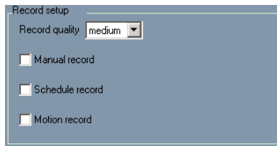
Fig 7.27 Record setup
