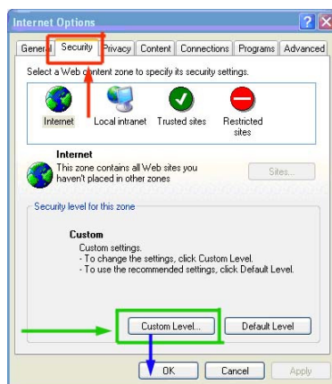
Fig 7.7 Internet Options
