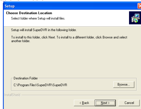
Figure3-10Select Installation Folder
