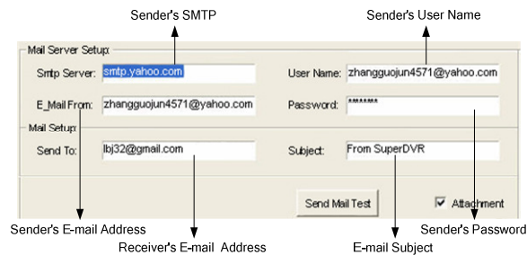
Figure5-13Auto Mail Setup
