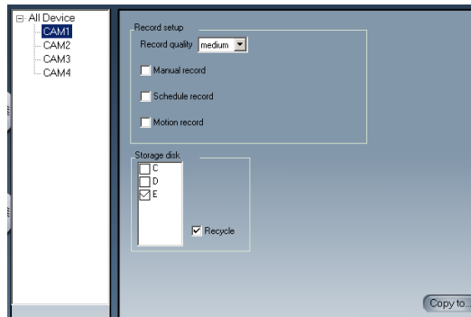
Fig 7.26 Record configuration
