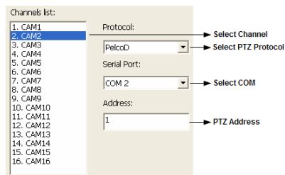
Figure5-18P.T.Z Protocol Setup
