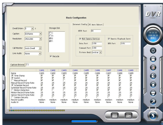
Figure5-1 Basic Configuration
