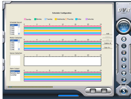
Figure5-7 Schedule Configuration
