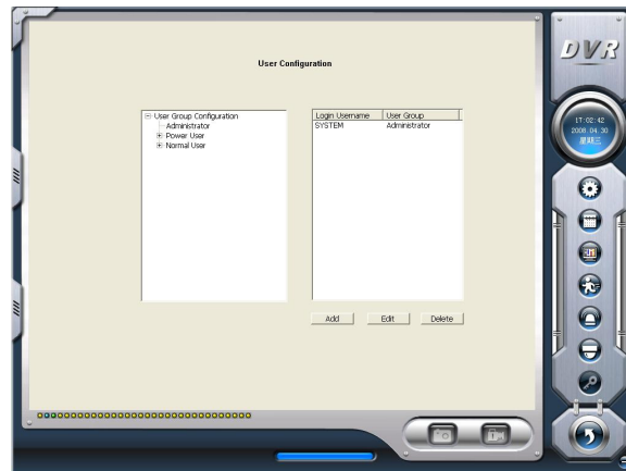
Figure5-20 User configuration
