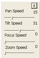
Figure6-3 Speed Adjustment
