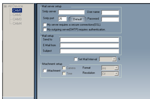
Fig 7.30 Email configuration
