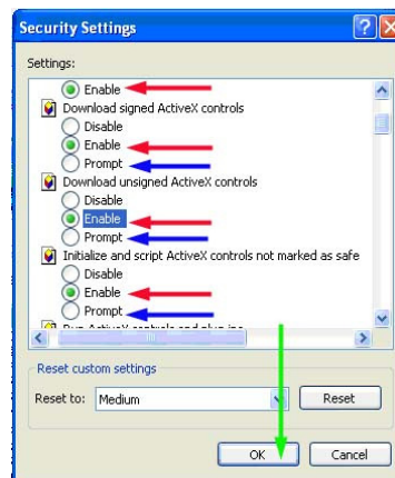
Fig 7.8 Security Settings
