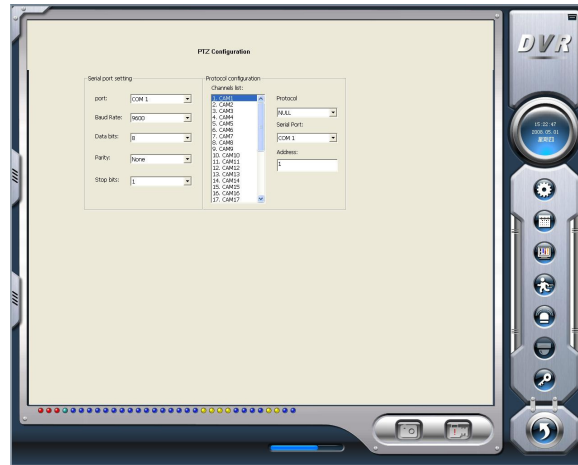
Figure5-17PTZ Configuration Panel
