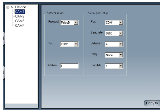
Fig 7.34 P.T.Z Configuration
