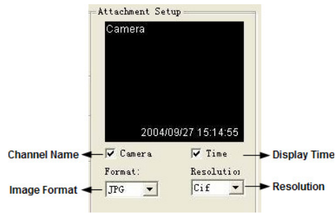
Figure5-14 Attachment Setup
