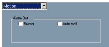
Fig 7.25 Alarm configuration
