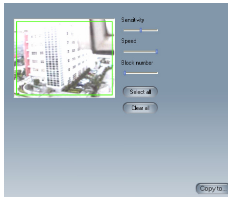
Fig 7.29 Motion configuration
