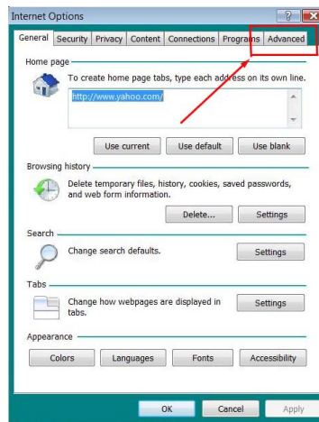
Fig 7.9 Advanced Options
