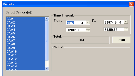
Figure7-12Delete Recorded Files
