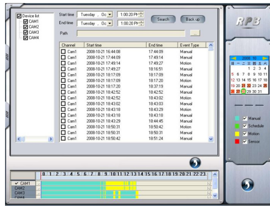
Fig 7.15 Remote backup
