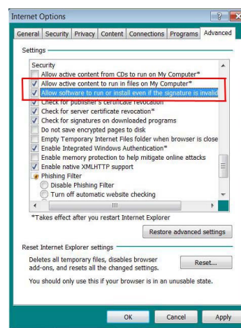
Fig 7.10 Invalid Signature
