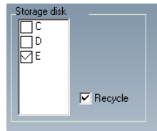
Fig 7.28 Storage disk
