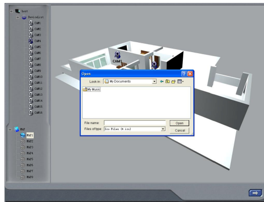
Figure5-15E-Map Edit
