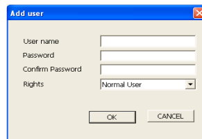
Figure5-22 Add User
