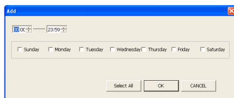
Figure5-8 Edit Schedule
