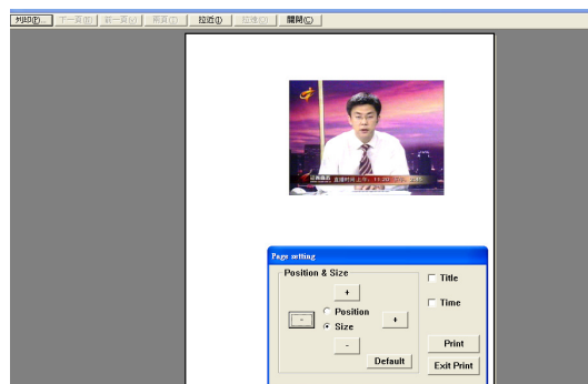
Figure7-16Print Preview
