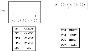
Figure2-2 Pins Definitions of QSDT8PCRC Video Capture Card
