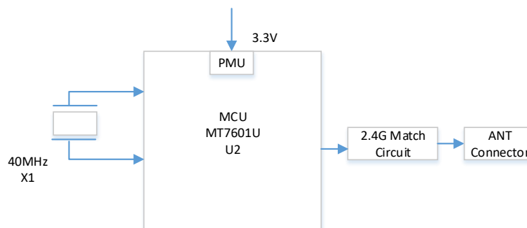
BLOCK DIAGRAM
