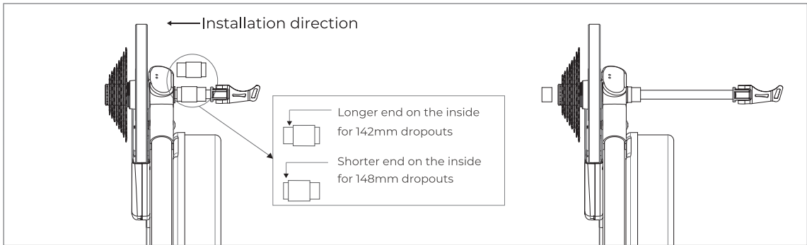
Fig 3 Axle installation
