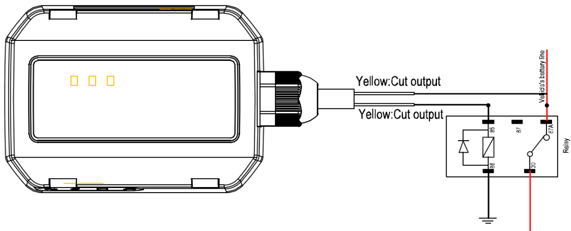
Figure 7. Typical Connection with Relay
