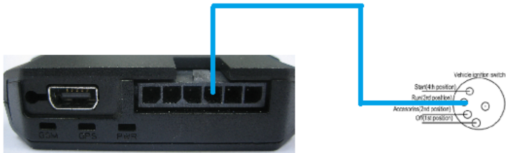
Figure 7. Typical Ignition Detection
