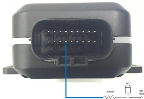
Figure 11. Typical Connection with a LED
