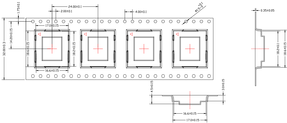
Figure 49: Dimensions of Tape
