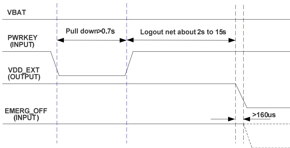
Figure 10: Turn-off Timing
