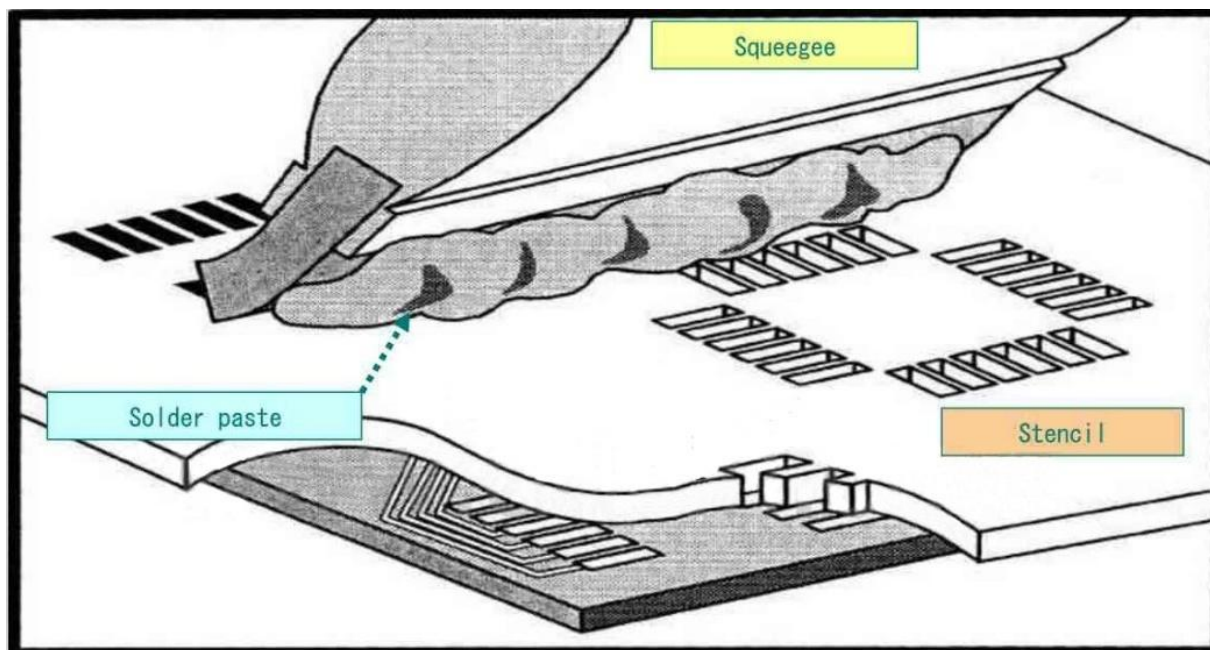
Figure 47: The Picture of Printing Paste
