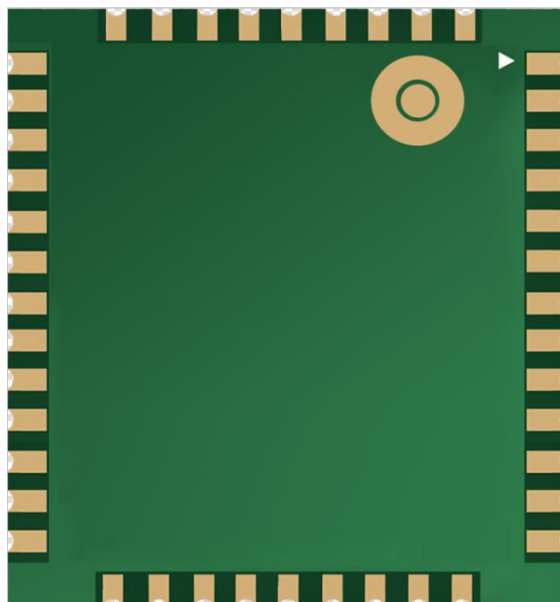
Figure 46: Bottom View of the Module
