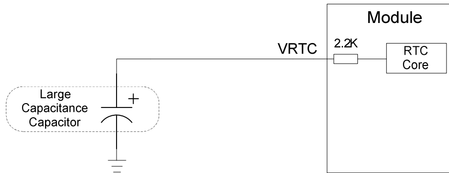
Figure 17: RTC Supplied from a Capacitor
