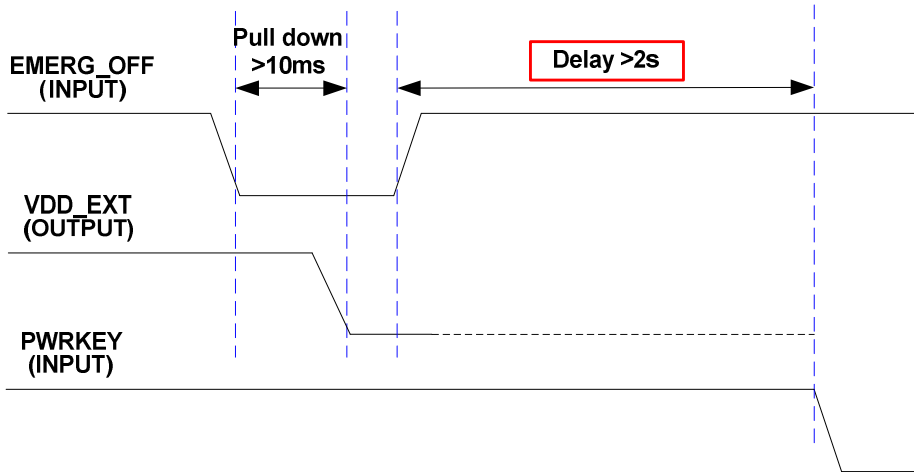
Figure 14: Timing of Restarting System after Emergency Shutdown
