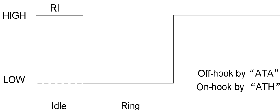
Figure 36: RI Behaviour of Voice Calling as a Receiver
