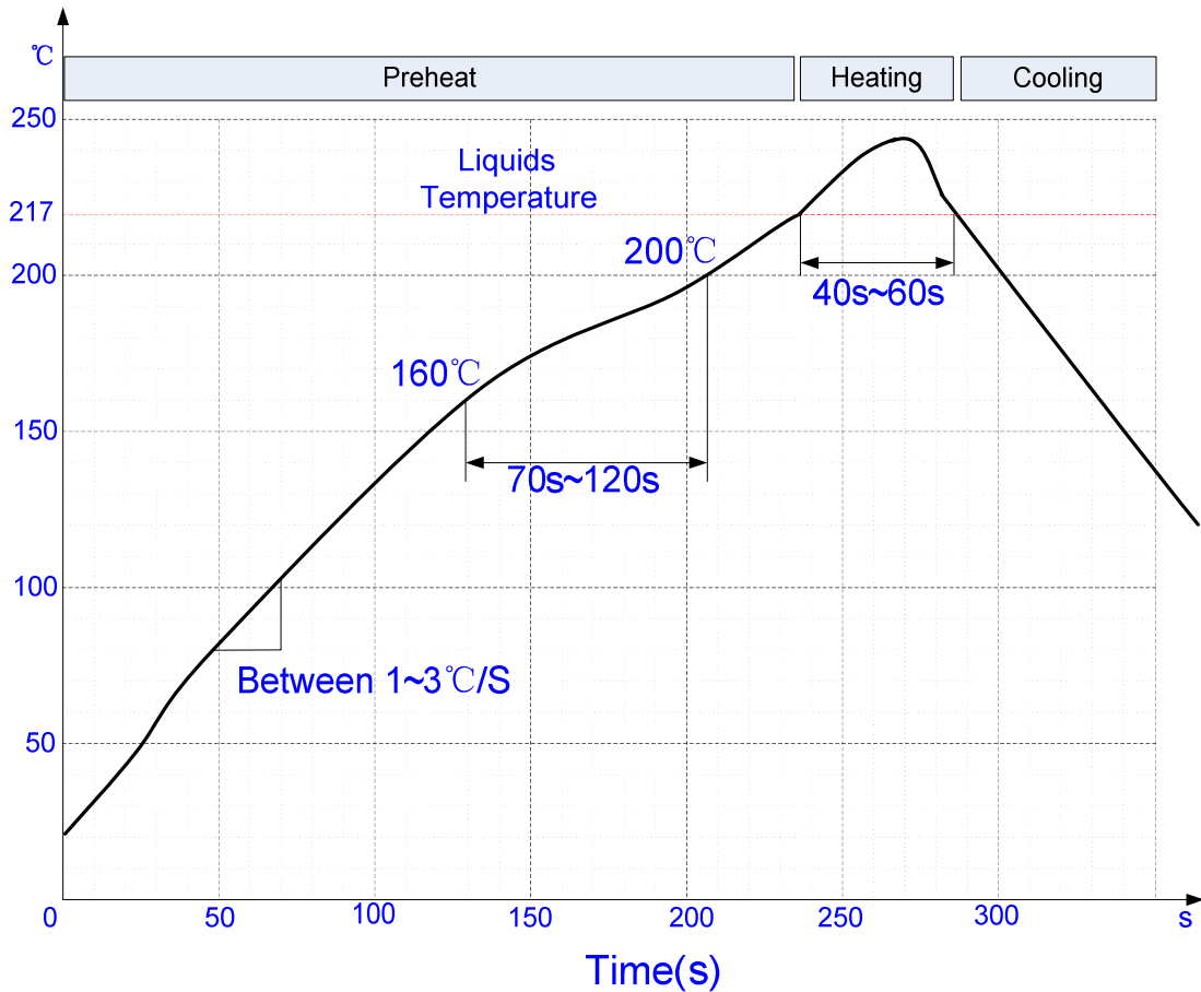
Figure 48: Ramp-Soak-Spike Reflow Profile
