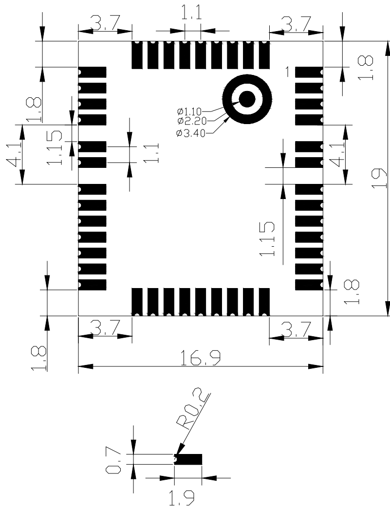
Figure 43: GC65 Module Bottom Dimensions (Unit: mm)
