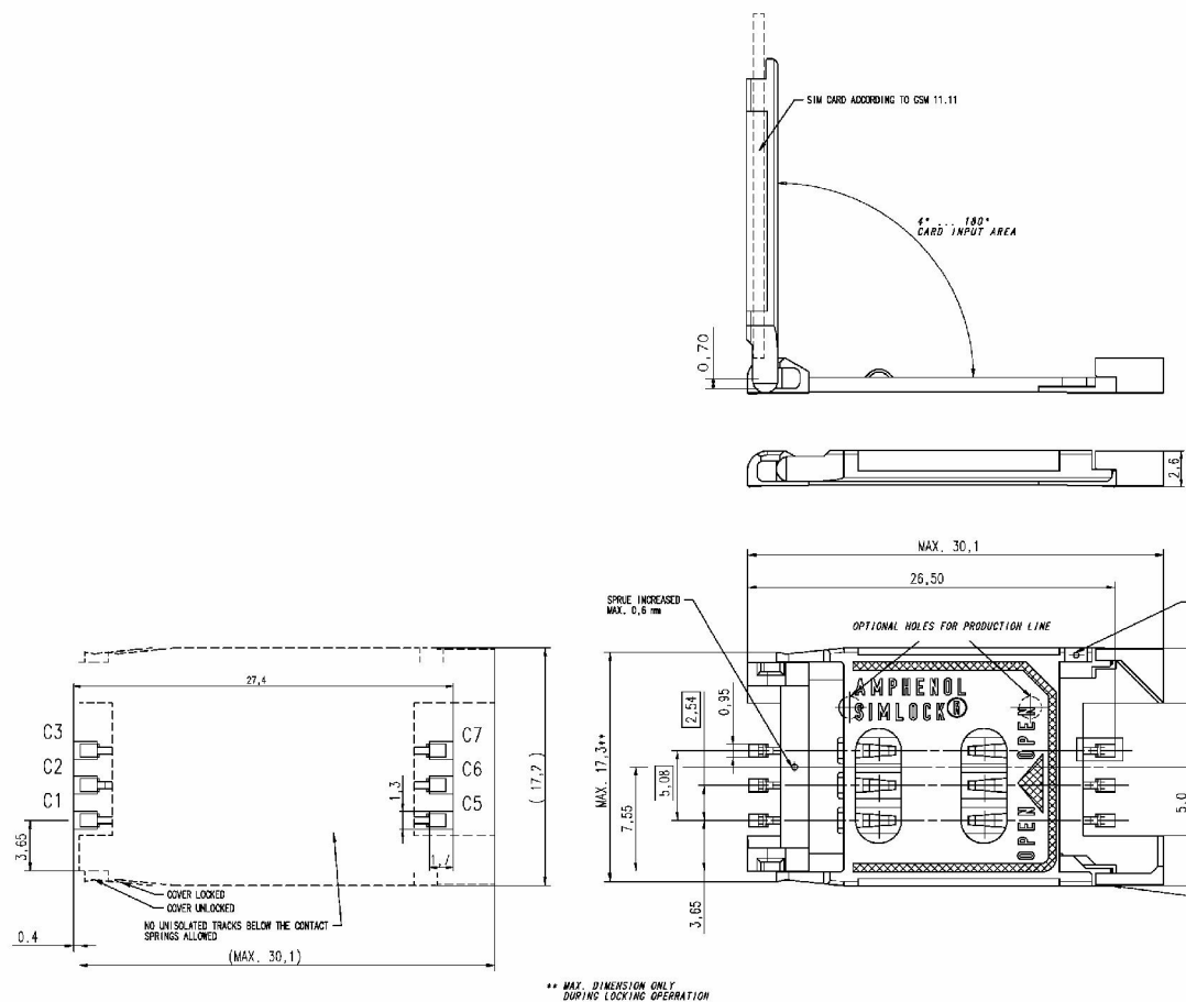
Figure 34: Amphenol C707 10M006 512 2 SIM Card Holder
