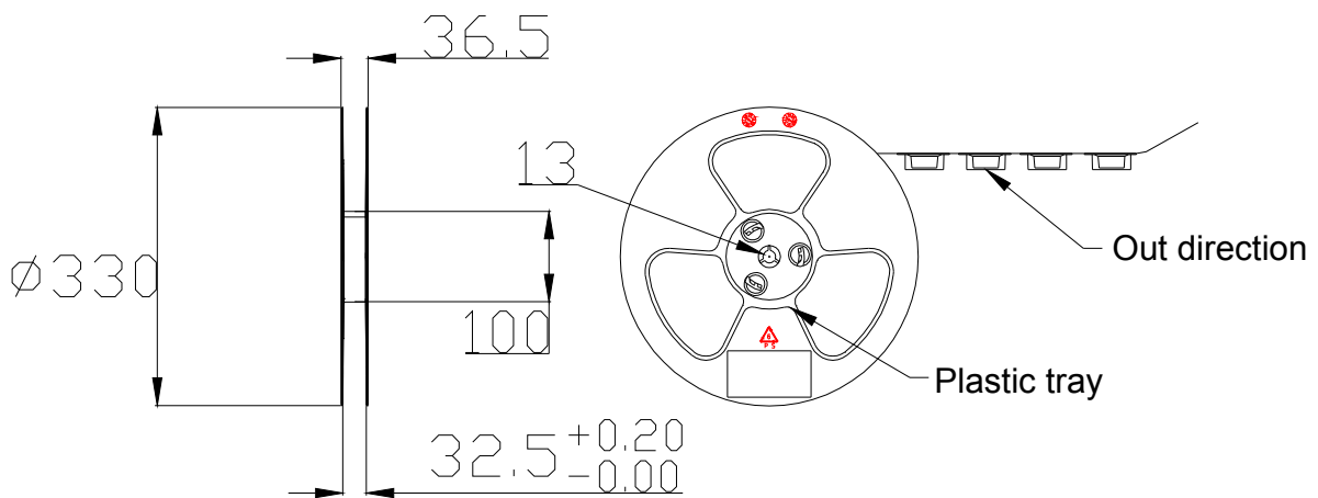
Figure 50: Dimensions of Reel
