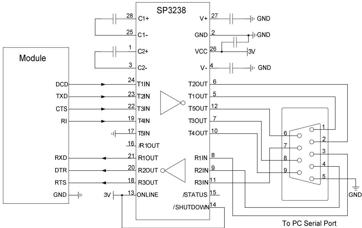
Figure 25: Level Match Design for RS-232
