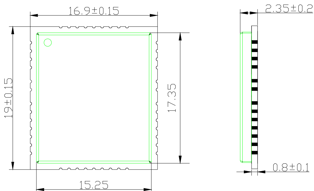
Figure 42: GC65 Module Top and Side Dimensions (Unit: mm)
