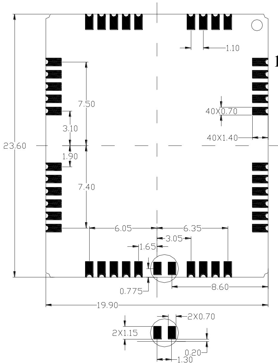
Figure 44: M35 Module Bottom Dimensions (Unit: mm)
