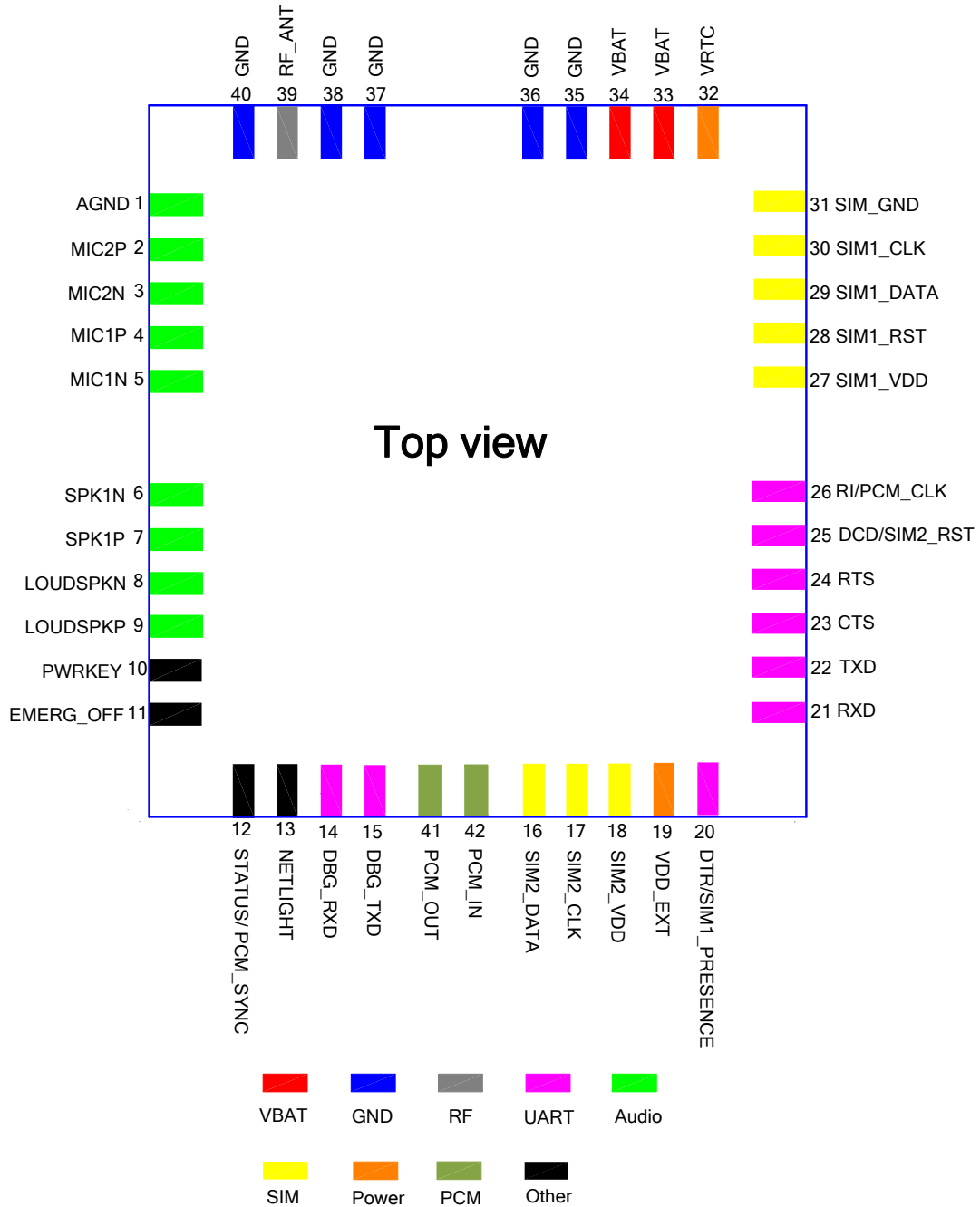
Figure 2: Pin Assignment
