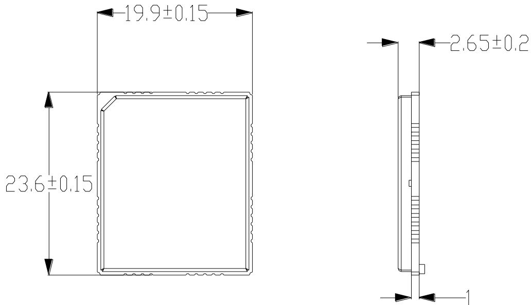
Figure 43: M35 Module Top and Side Dimensions (Unit: mm)
