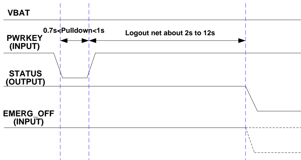
Figure 9: Turn-off Timing
