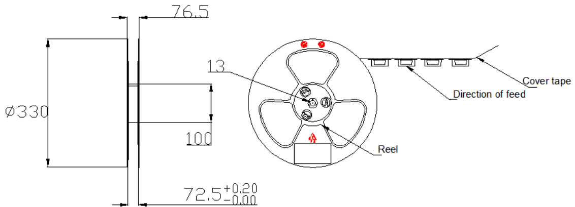
Figure 26: Reel Dimensions
