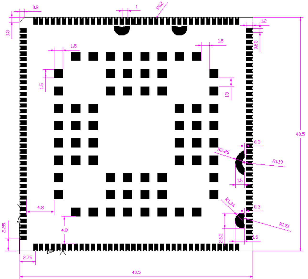
Figure 19: Module Bottom Dimensions (Top View)
