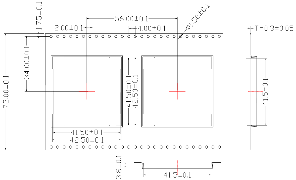
Figure 25: Tape Dimensions
