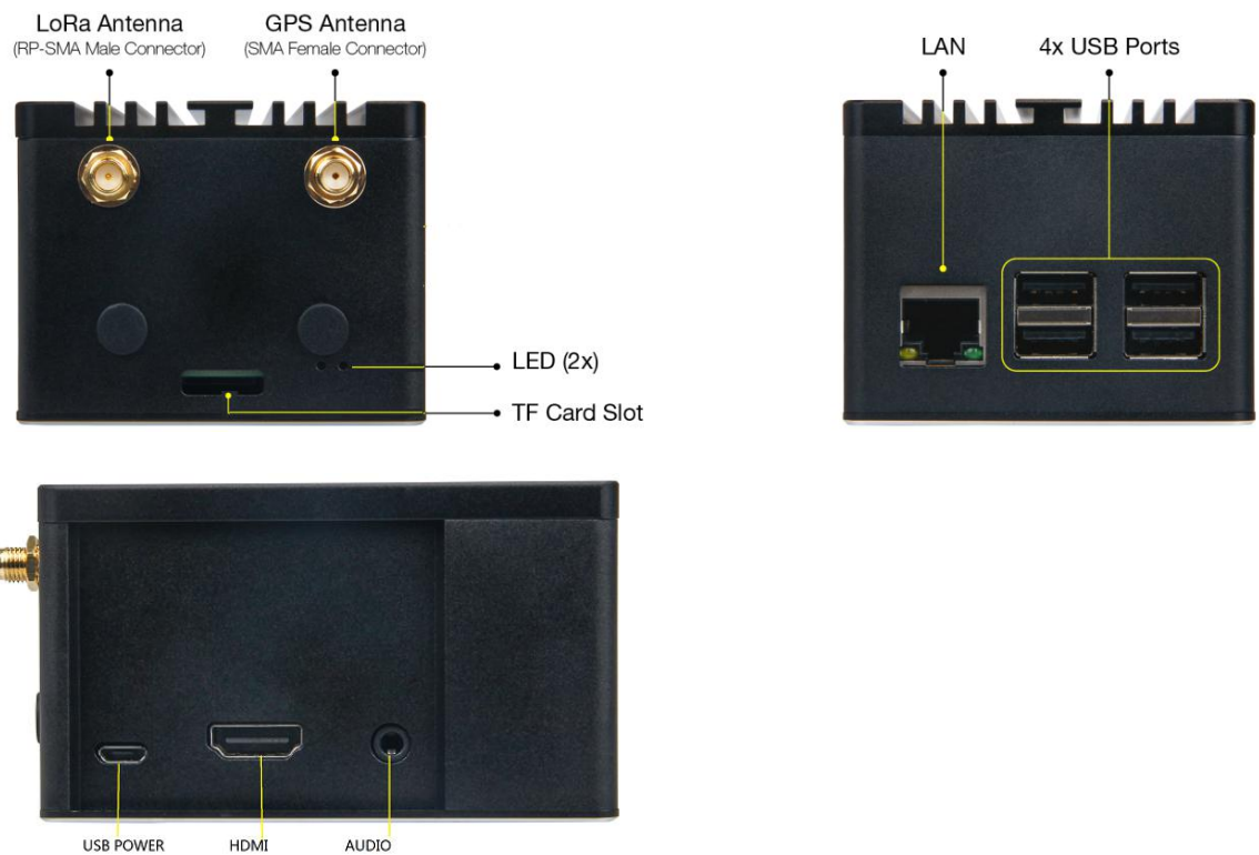
Figure 3 | Interfaces
