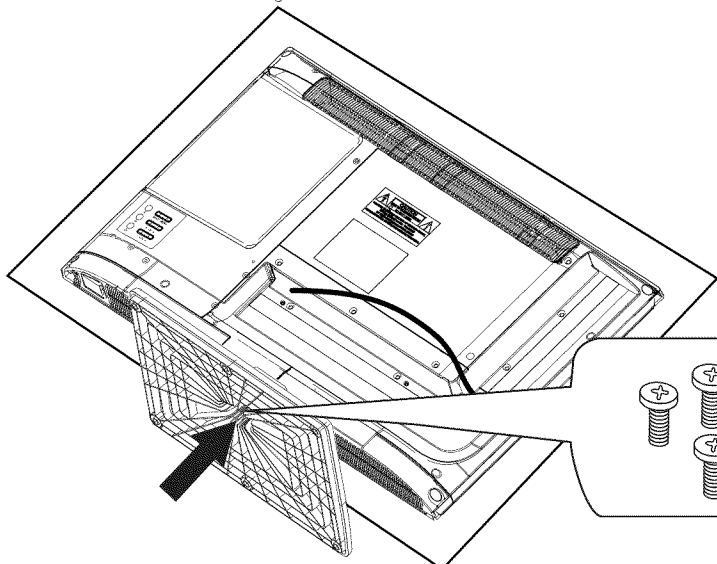
The bottom view of the TV (Front cabinet faces down)
