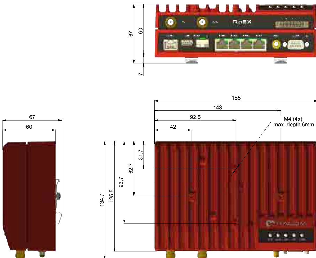
Fig. 2.1: RipEX2 dimensions
