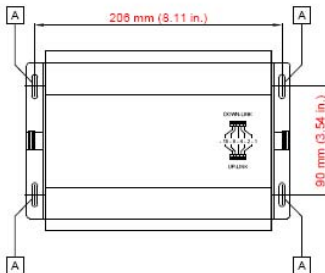
FIGURE 2 – POSITION OF THE PRE-CUT SLOTS
