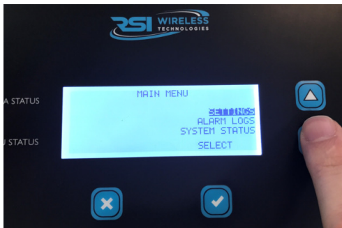
Figure 3 – Main Menu
