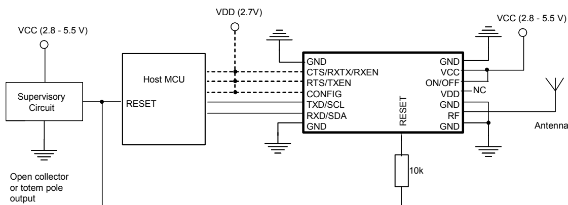
Figure 4. Reset circuit using supervisory circuit on VCC
