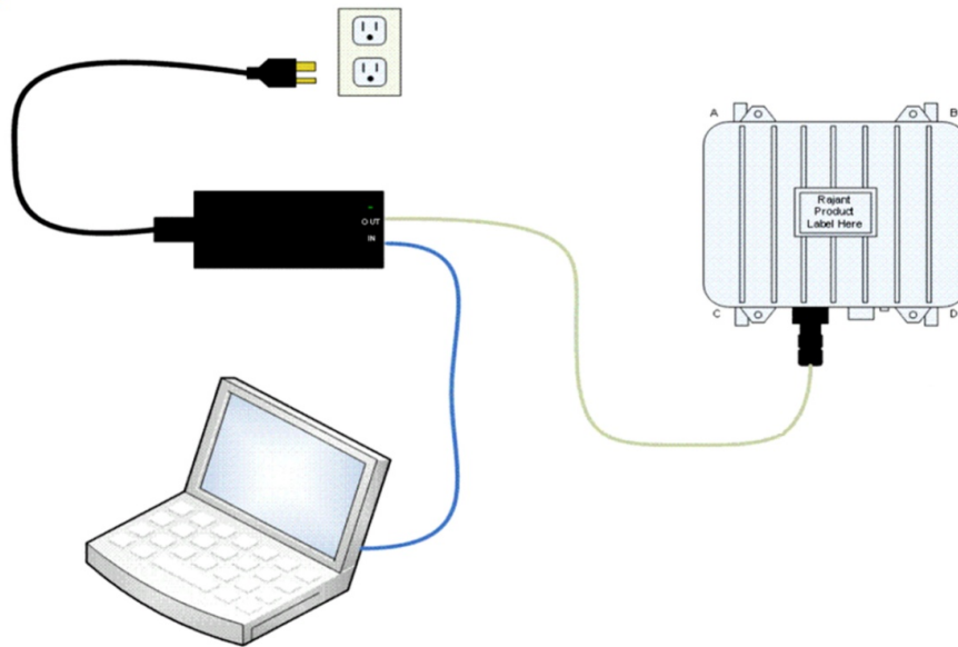
Figure 5: BreadCrumb LX/LX3 Ethernet and Passive PoE Connections.
