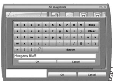
Figure 11-1: On-screen keyboard
