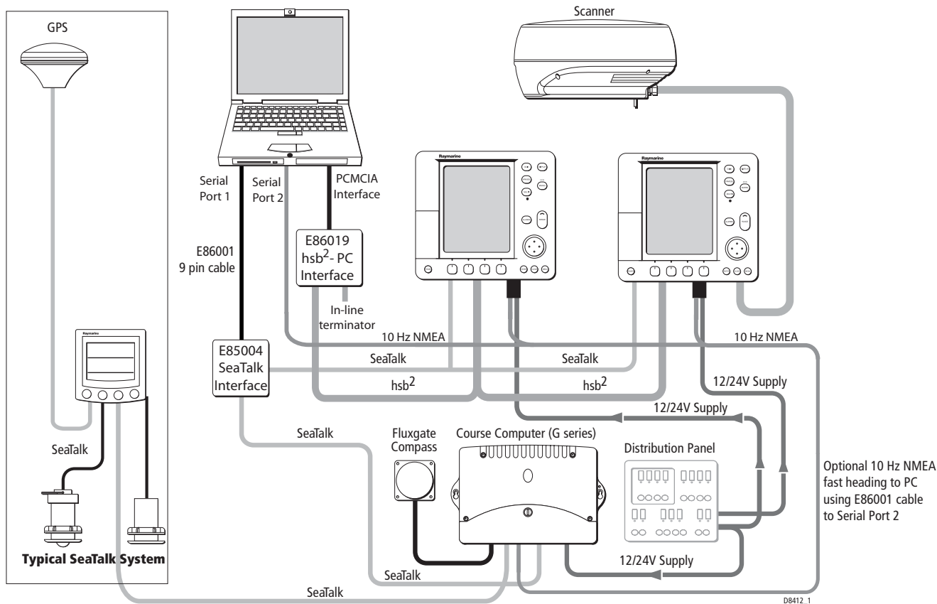
Fully integrated hsb 2 system
