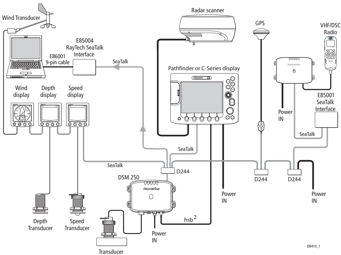
Raymarine SeaTalk system
