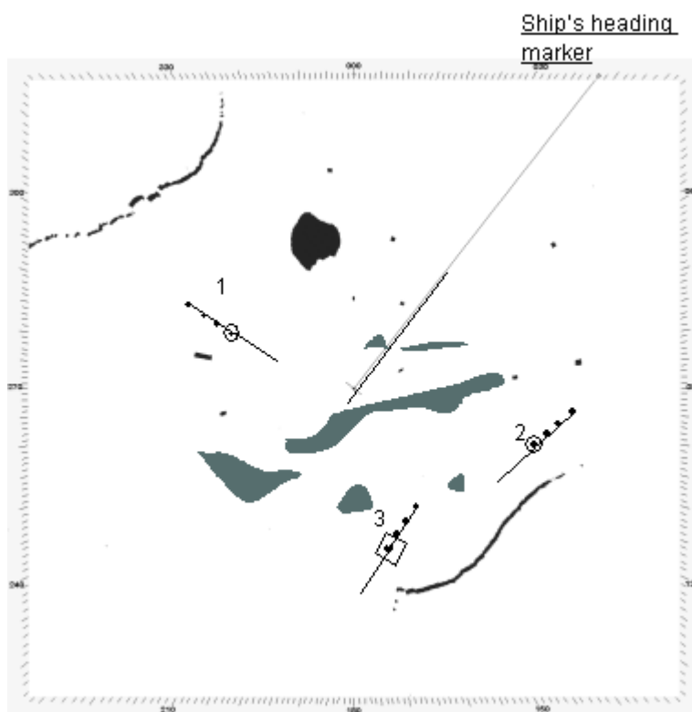
Figure 3-11 Relative Vector Mode
