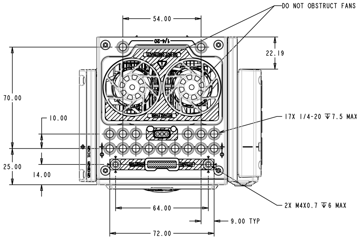
Figure: EPIC-W 5K S35 Top View
