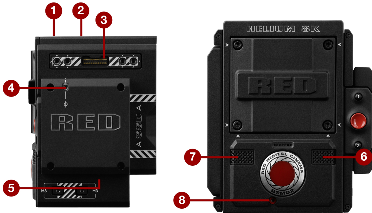
Figure: DSMC2 HELIUM Ports and Features
