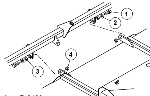
Asm-R-0108
