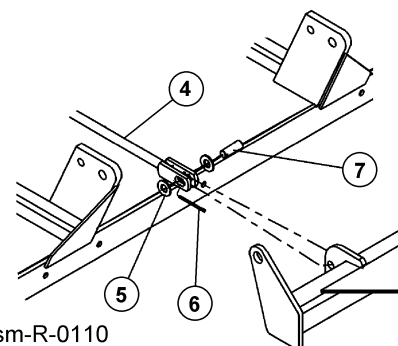
Asm-R-0110
