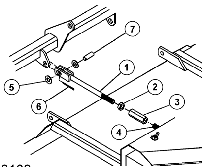
Asm-R-0109
