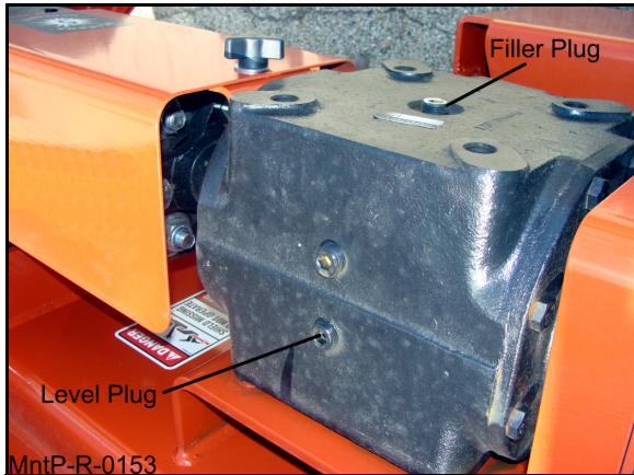
Center Gearbox
