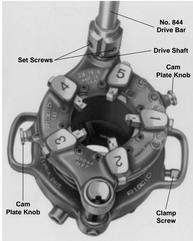
Figure 7 – No. 141 Geared Threader (No. 161 Threader Similar)
