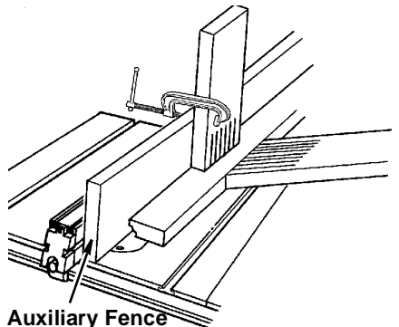
Auxiliary Fence
