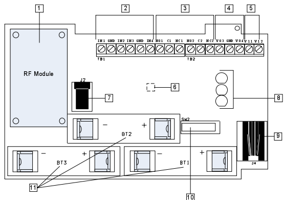
Figure 1: Wireless I/O Module Main Components
