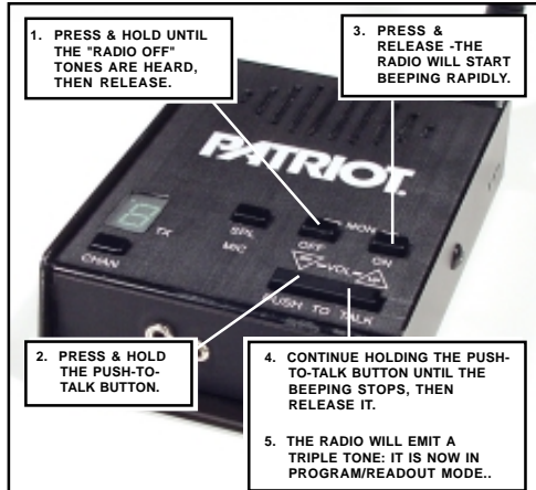
FIG-5: HOW TO PLACE THE RADIO IN PROGRAM/READOUT MODE
