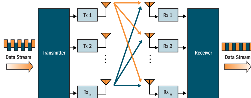
Figure 18. Spatial Multiplexing
