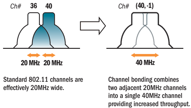
Figure 19. Channel Bonding
