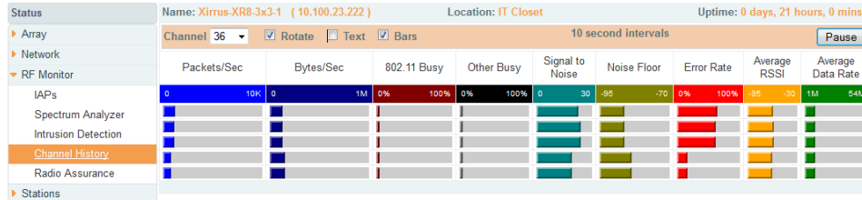
Figure 66. RF Monitor—Channel History (Rotated)
