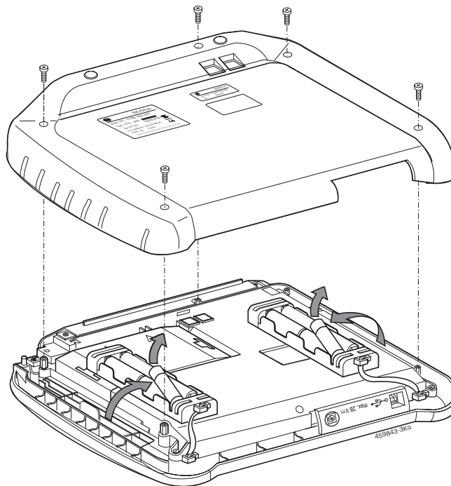
Fig. 4: Battery replacement
