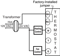
HEAT ONLY 3-WIRE SINGLE TRANSFORMER
