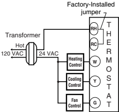
HEAT/COOL 4-WIRE SINGLE TRANSFORMER
