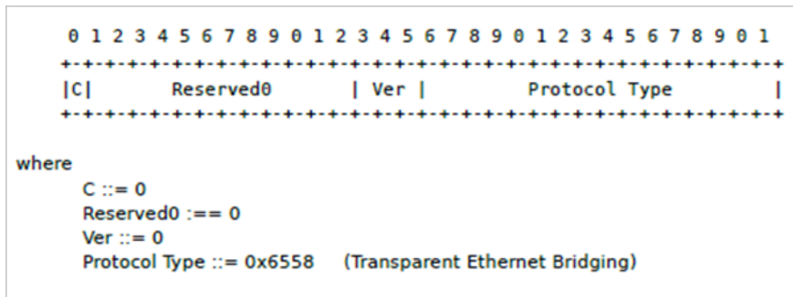
Figure 7: L2oGRE header
