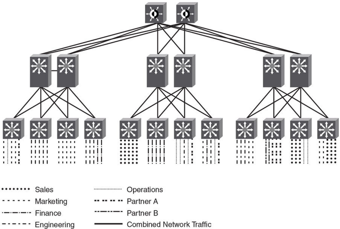
FIGURE 38 Example high-level Multi-VRF topology
