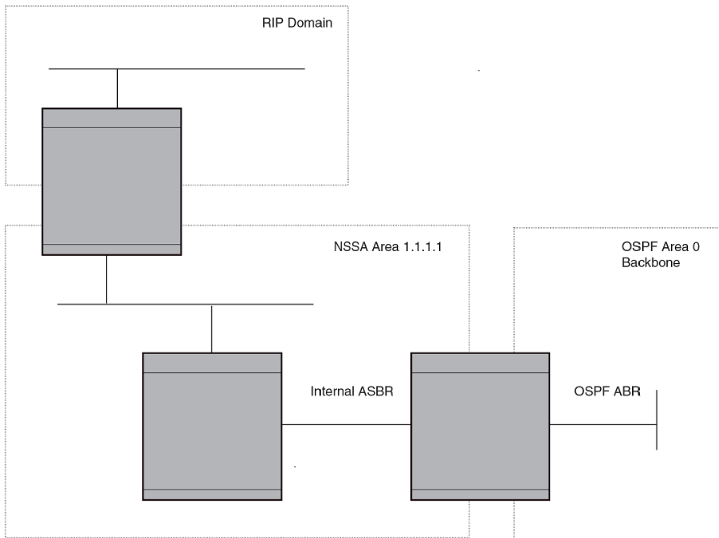
FIGURE 22 OSPF network containing an NSSA
