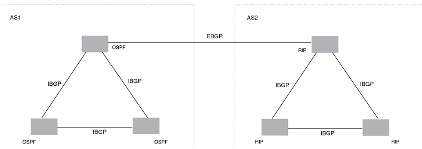
FIGURE 29 Example of customer connected to two ISPs
