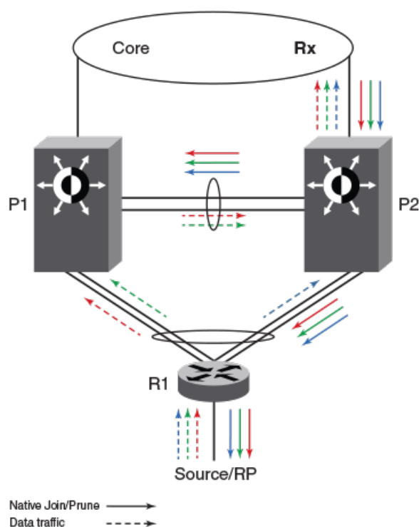
FIGURE 46 MCT peer as immediate downstream router
