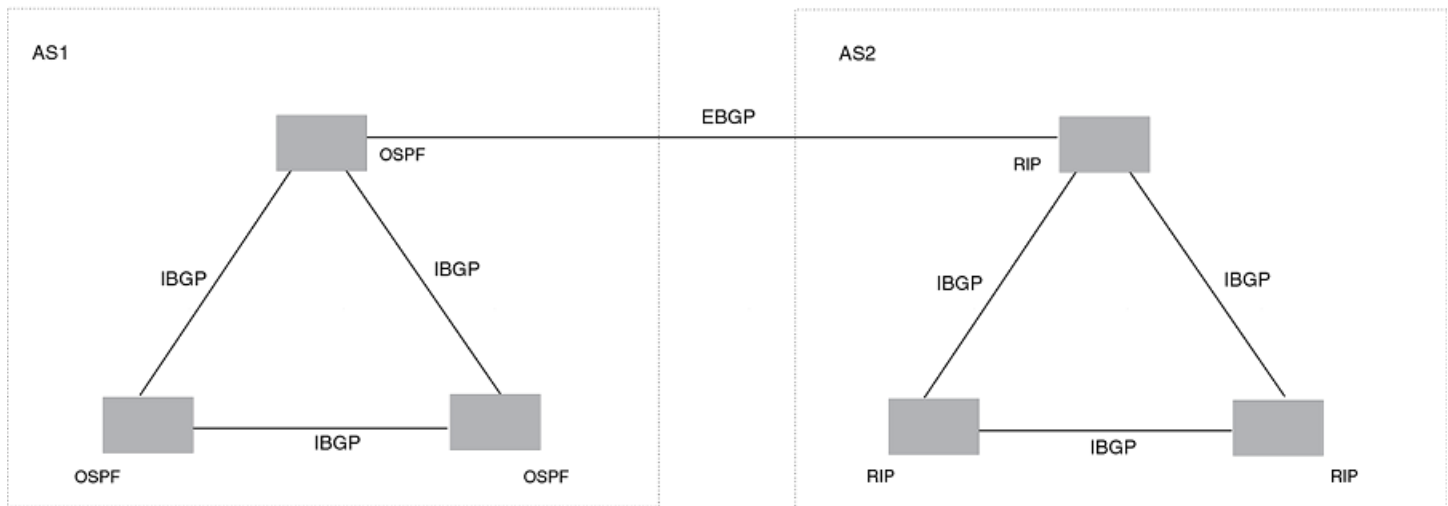
FIGURE 27 Example BGP4 autonomous systems
