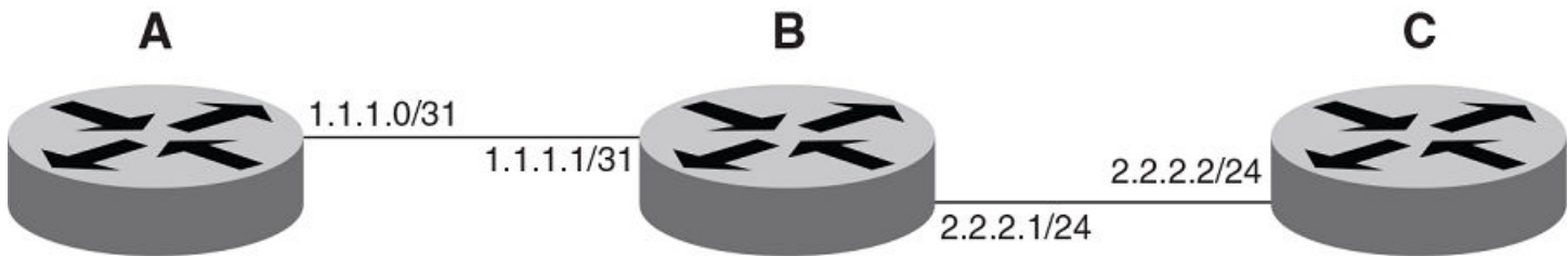
FIGURE 2 Configured 31-bit and 24-bit subnet masks
