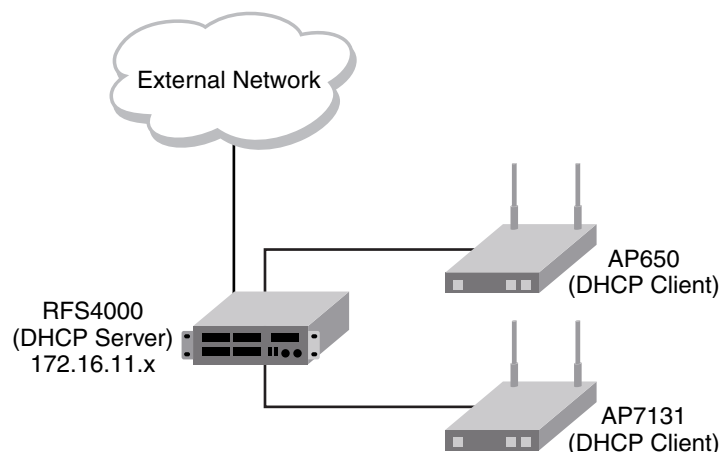
FIGURE 1 Network Design
