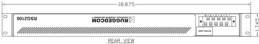
REAR VIEW
