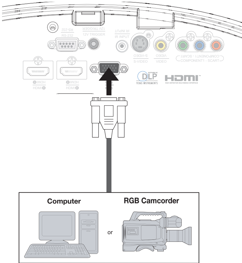
Figure 3-9. RGB Connections
