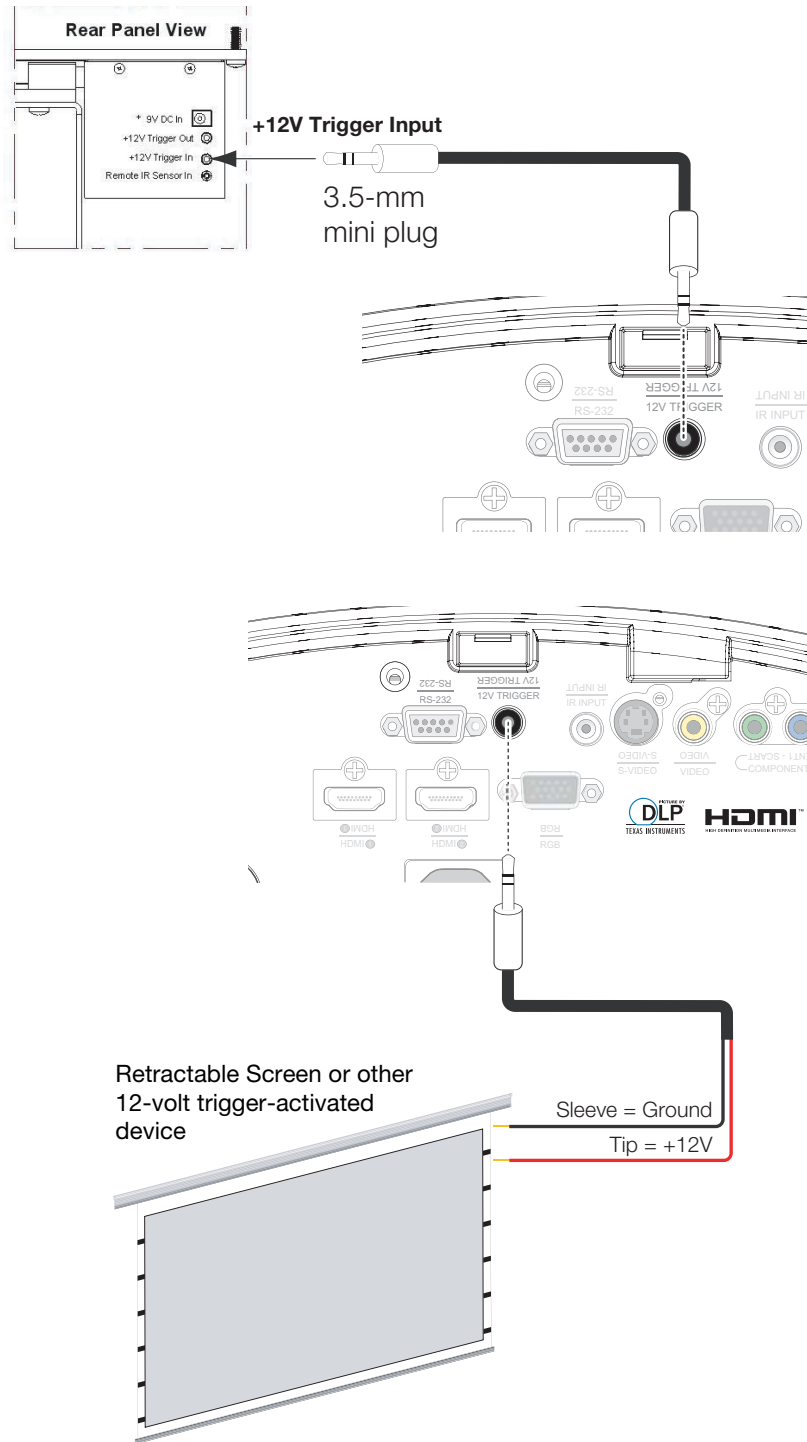
Figure 3-14. 12-Volt Trigger Output Connection
