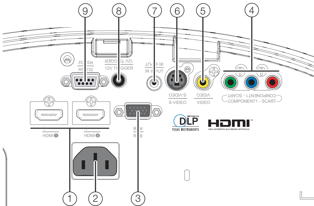
Figure 2-3. LS-1 Rear Panel
