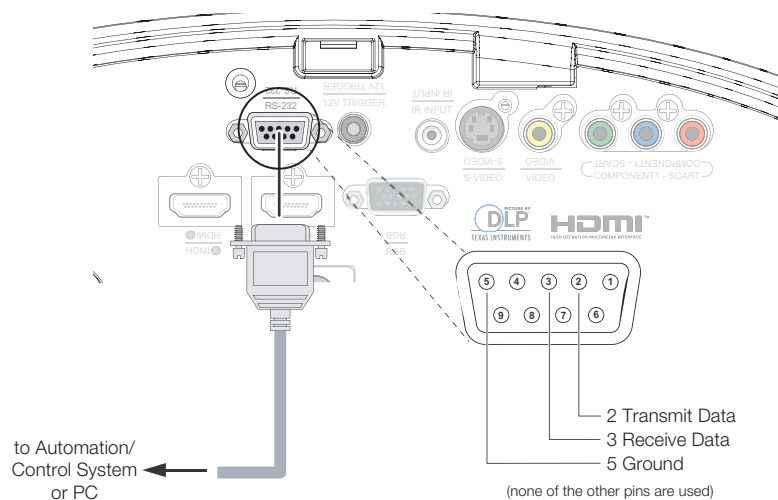
Figure 3-13. RS-232 Control System Connection
