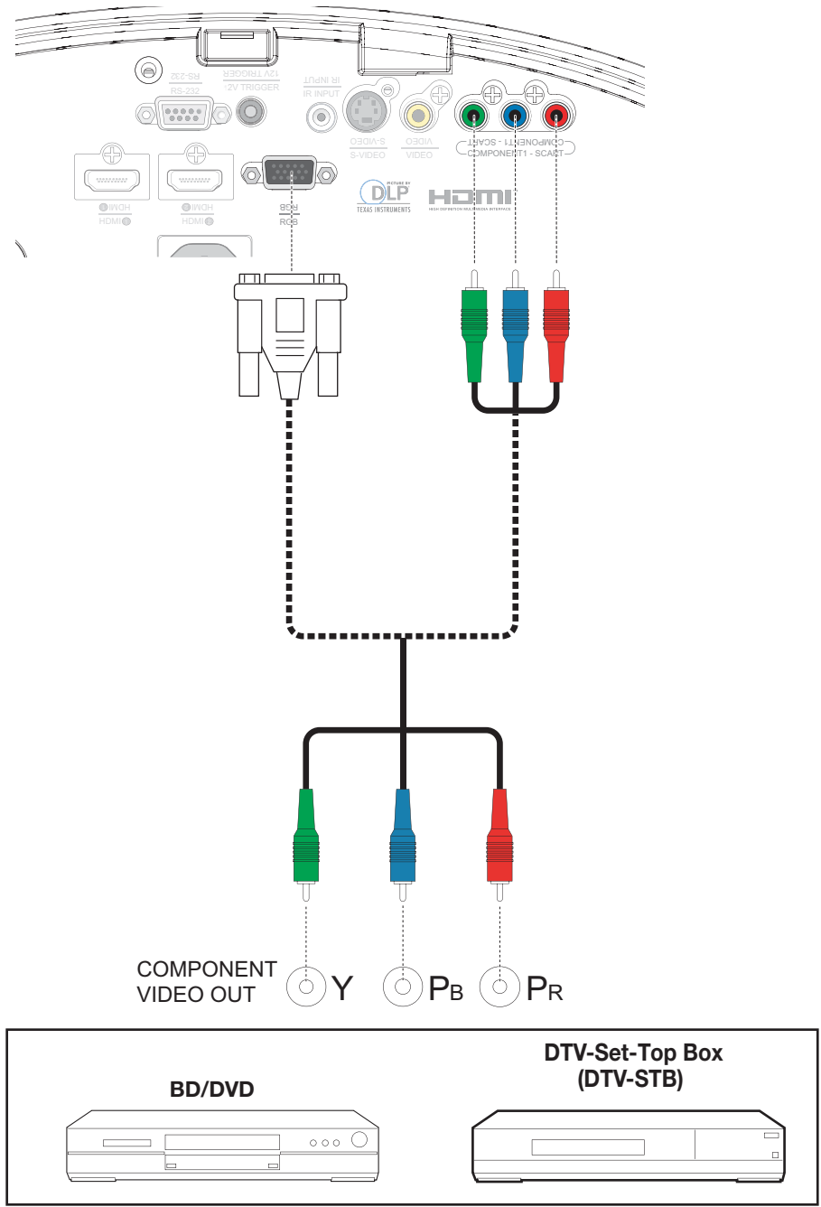
Figure 3-11. Component Video Connections
