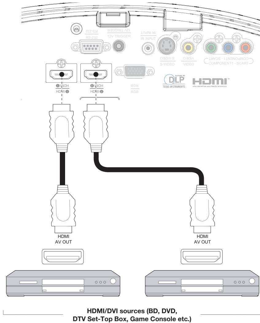
Figure 3-8. HDMI/DVI Source Connections
