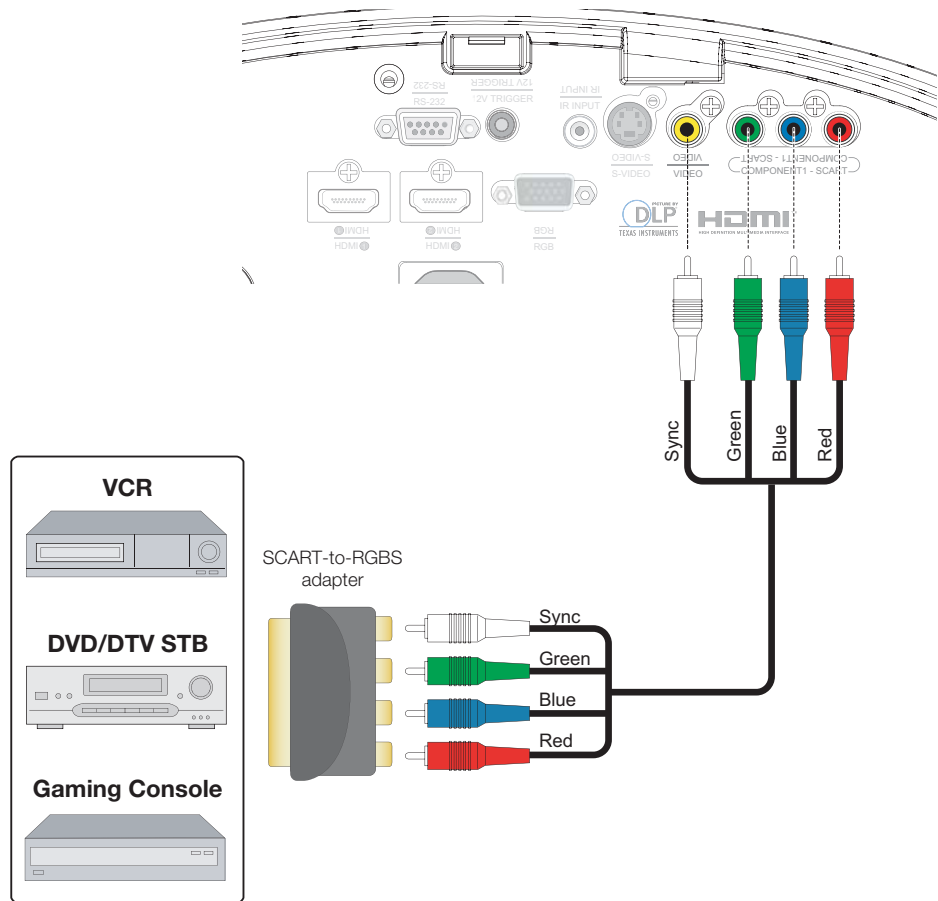
Figure 3-10. SCART RGBS Connection
