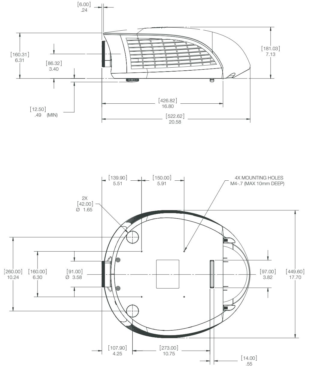
Figure 7-1. LS-1 Dimensions
