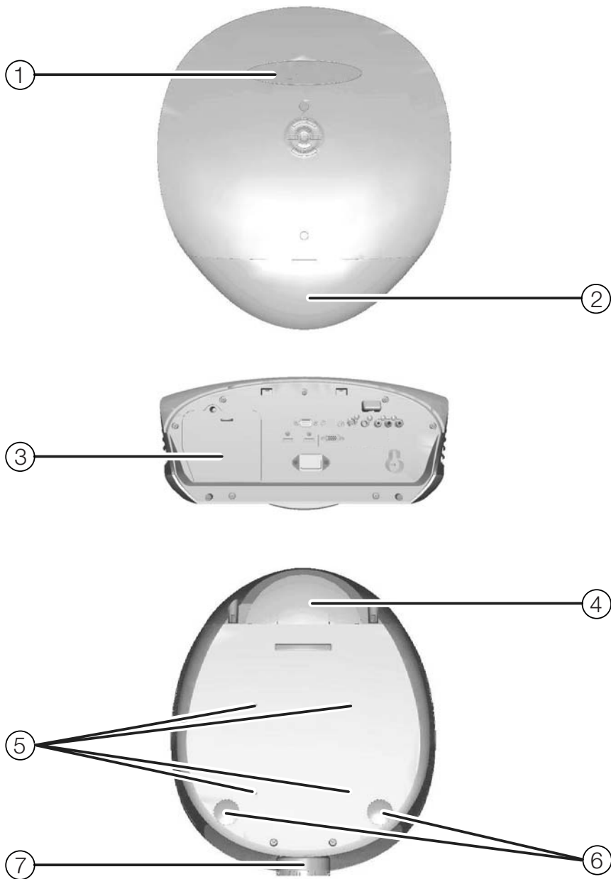
Figure 2-2. LS-1 Rear/Bottom/Top View
