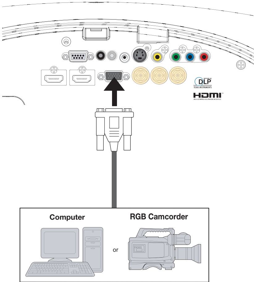
Figure 3-9. RGB Connections
