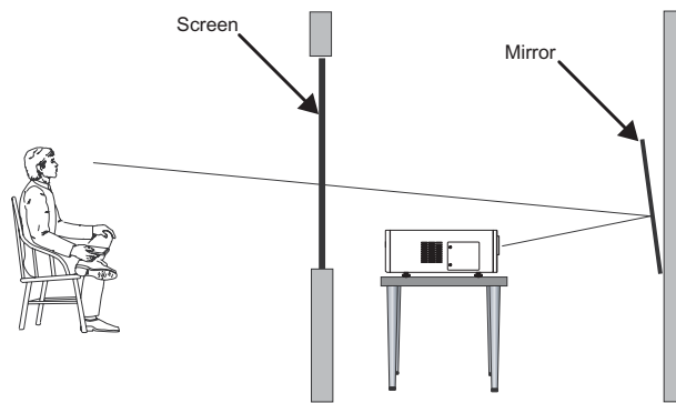
Figure 3-5. Folded Optics
