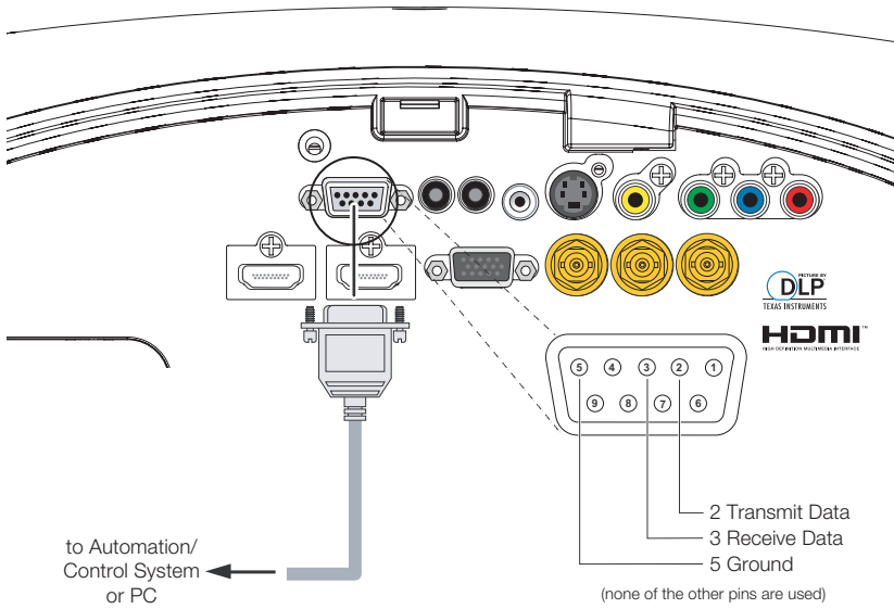
Figure 3-13. RS-232 Control System Connection
