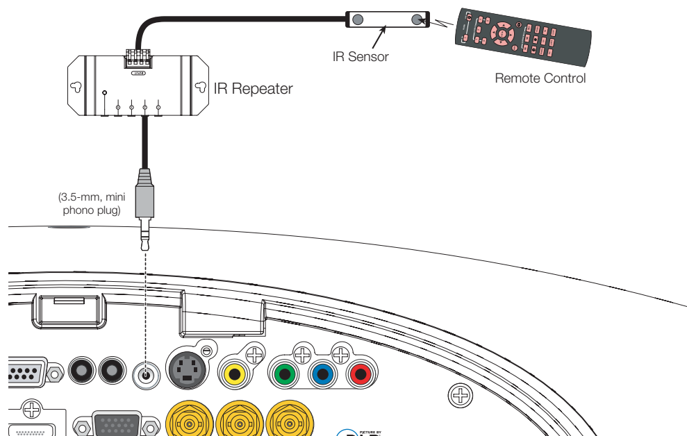
Figure 3-15. External IR Receiver Connection
