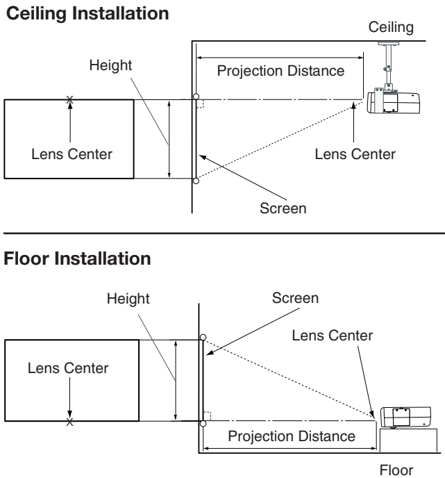
Figure 3-3. Projector Placement
