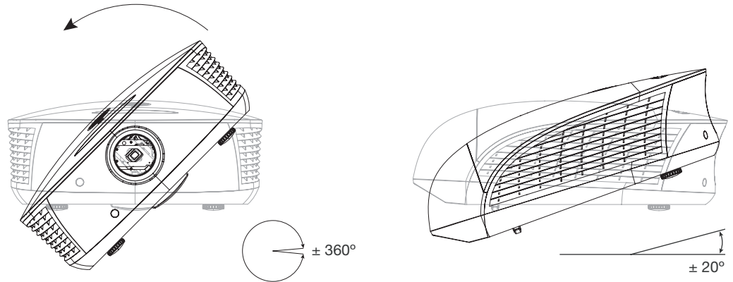
Figure 3-7. Mounting Angle Ranges (Side-to-Side and Front-to-Back)
