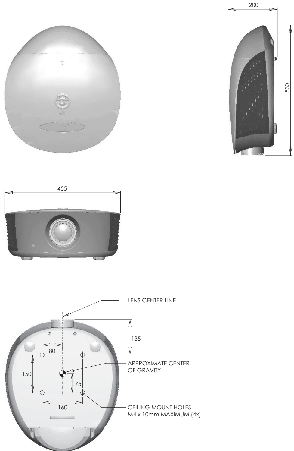
Figure 7-1. LS-HB Dimensions
