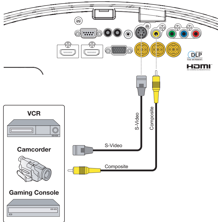
Figure 3-12. Composite and S-Video Connections
