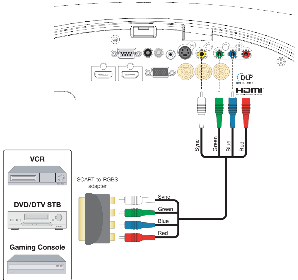
Figure 3-10. SCART RGBS Connection
