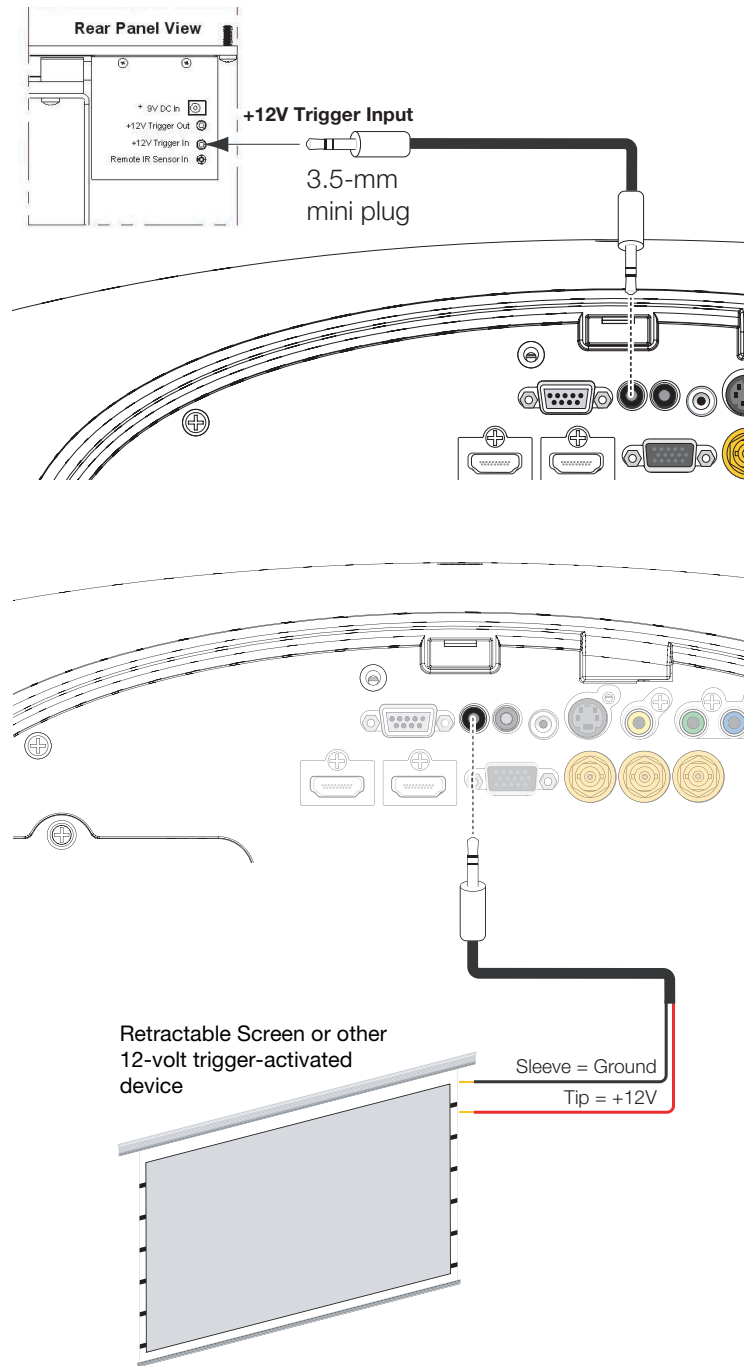
Figure 3-14. 12-Volt Trigger Output Connection
