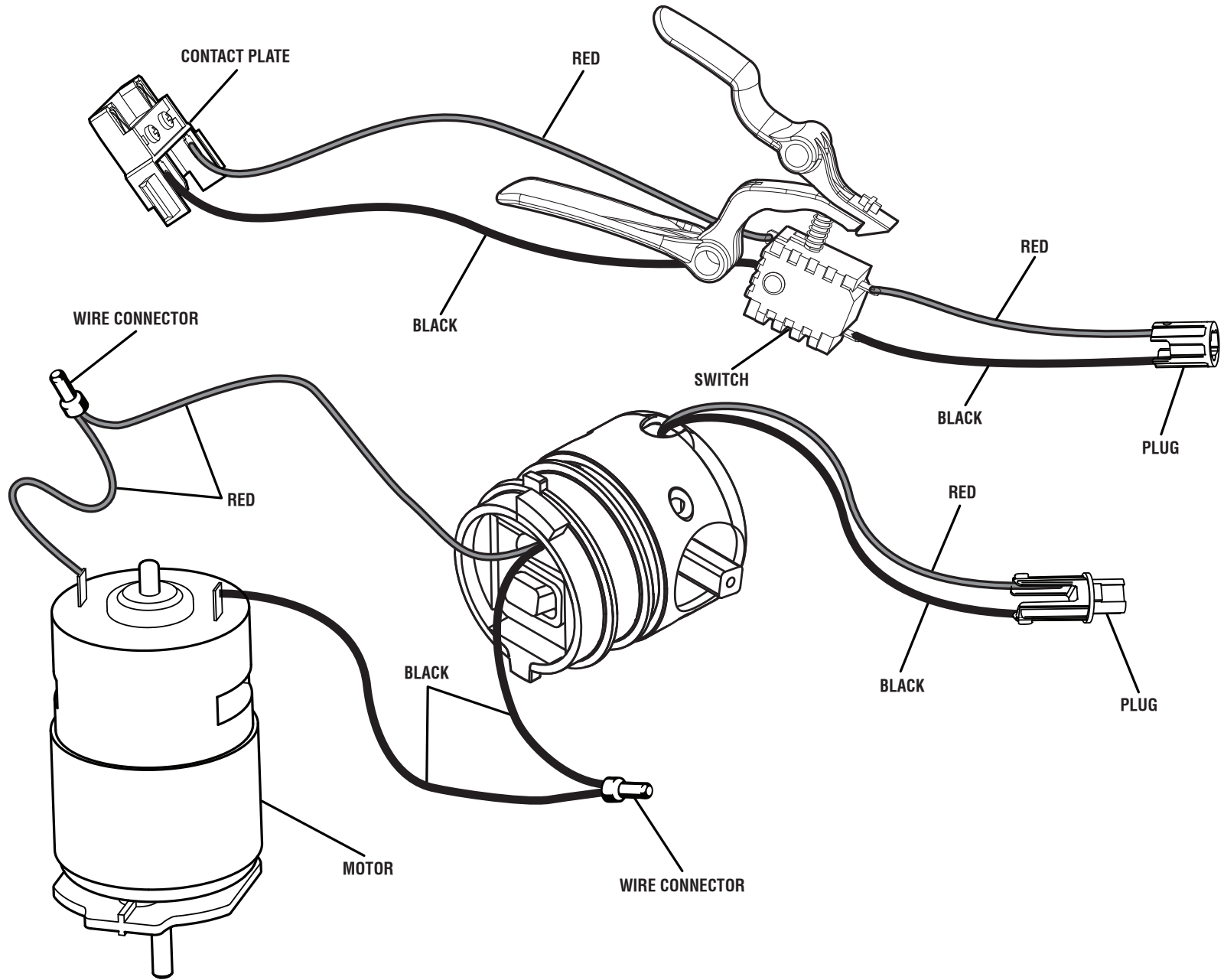
WIRING DIAGRAM
