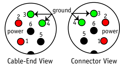
FIGURE 3.2 S&C IntelliCom WAN 1720 DC Connector
