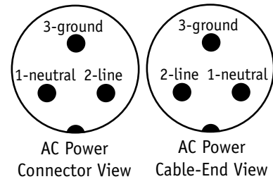
FIGURE 3.1 S&C IntelliCom WAN 1720 AC Connector
